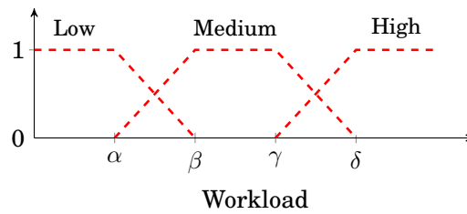
Fig. 3. Fuzzy membership functions for auto-scaling variables.
