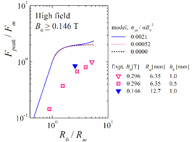
FIG. 10: High magnetic field ( B_0 \geq 0.146 \text{ T} ) comparison between measured peak adhesive force (symbols) and model predictions ( \sigma_{y0} = 6.24 \text{ Pa} , \alpha = 137737 \text{ Pa}\cdot\text{T}^{-2} ), for various initial geometries h_0 and (R_0/R_m) . The theoretical predictions of the current model are given by the lines (Eq. 14). No fitting parameters are used. The experimentally measured adhesive strength is systematically lower than predicted by theory for these large field strengths.
