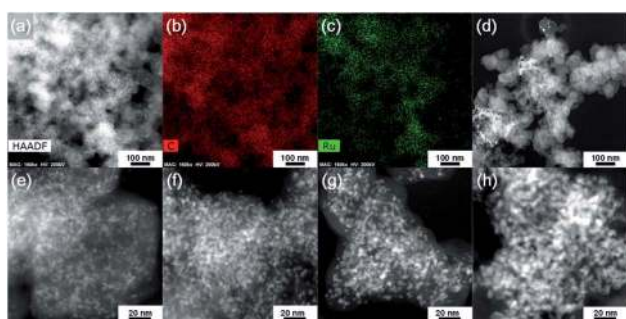
Fig. 3 (a) HAADF-STEM image of the Ru catalyst with 30 cycles (~32 wt%) synthesized by FBR-ALD. TEM-EDS images of (b) C element and (c) Ru element, corresponding to (a). (d) HAADF-STEM images of the commercial Ru catalyst (Premetek, 20 wt%) and the FBR-ALD-synthesized Ru catalysts as a function of the number of ALD cycles: (e) 5 cycles, (f) 10 cycles, (g) 20 cycles and (h) 30 cycles.
