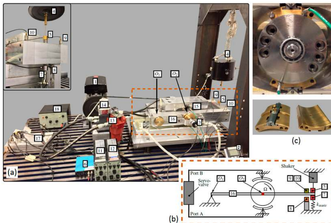
Figure 5. (a) Photo of the test bench with instrumentation: 1 AC motor and frequency converter; 2 Control unit for the frequency converter; 3 Tachometer; 4 Electromagnetic shaker; 5 Force transducer; 6 Amplifier for the force transducer; 7 Force transducer for the static load; 8 Displacement sensor; 9 and 10 Accelerometers; 11 and 12 Amplifiers for the accelerometers; 13 Oil filter; 14 Servo valve; 15 Pressure sensor (green wire); 16 Frame; 17 dSpace unit for signal acquisition; 18 Amplifier for the electromagnetic shaker; (b) dashed box containing the schematized rotor-lever system; (c) pair of instrumented tilting-pads dismantled and mounted on the rotor.
