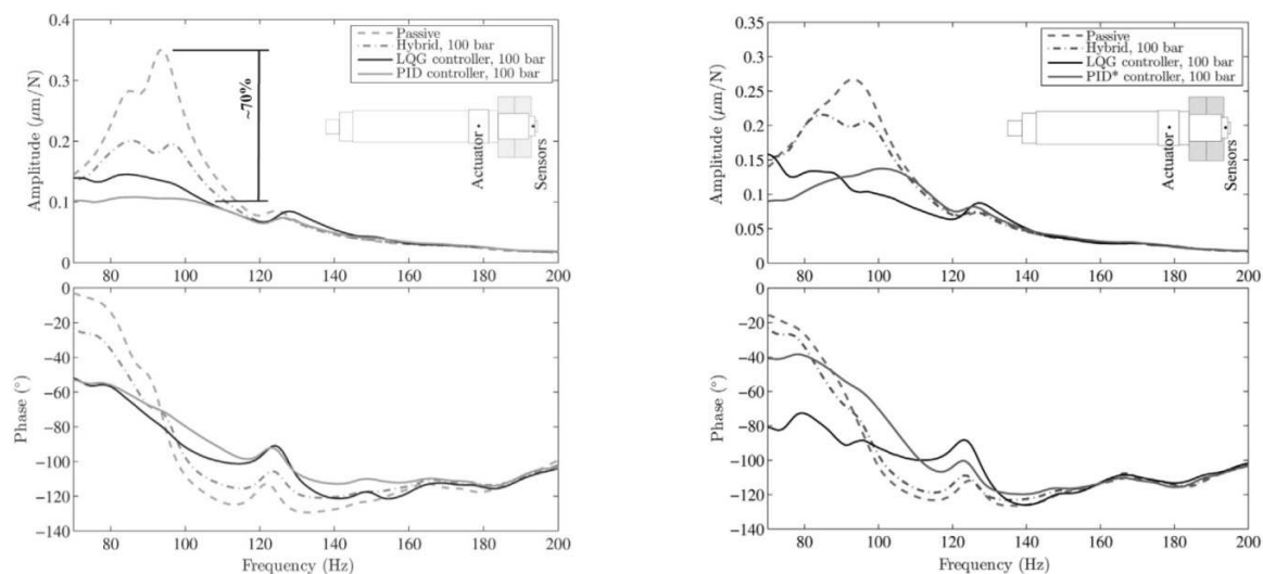
Figure 4. Horizontal and vertical lateral dynamics of the rotor–bearing system measured at the end of the shaft and excited by the electromagnetic shaker when four cases are investigated: hydrodynamic (conventional); hybrid using 100 bar; active using a LQG model-based controller; and active using an empirically-tuned PID controller [43]. Copyright from Elsevier.
