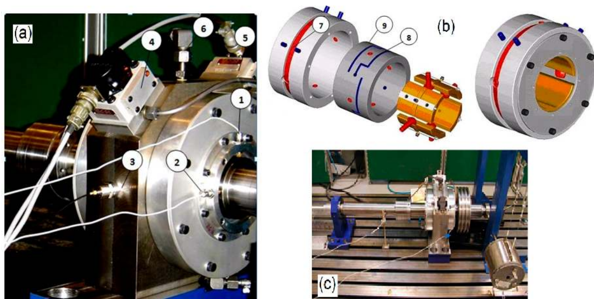
Figure 3. (a) Sliding bearing with incorporated sensing and actuation systems; (b) design solution and compactness; (c) test bench composed of a flexible rotor–disc excited by an electromagnetic shaker and controlled via active sliding bearing.
