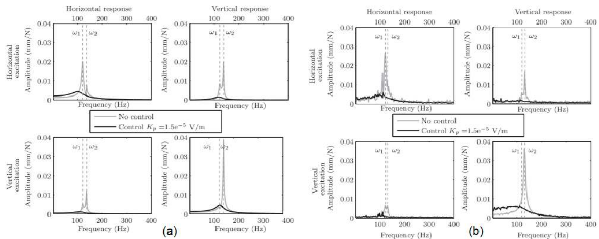
Figure 2. Theoretical and experimental frequency response of the rotating disc due to impulse excitations where the hybrid lubrication is illustrated in gray and the active lubrication in black: (a) theoretical results and (b) experimental results [39].
