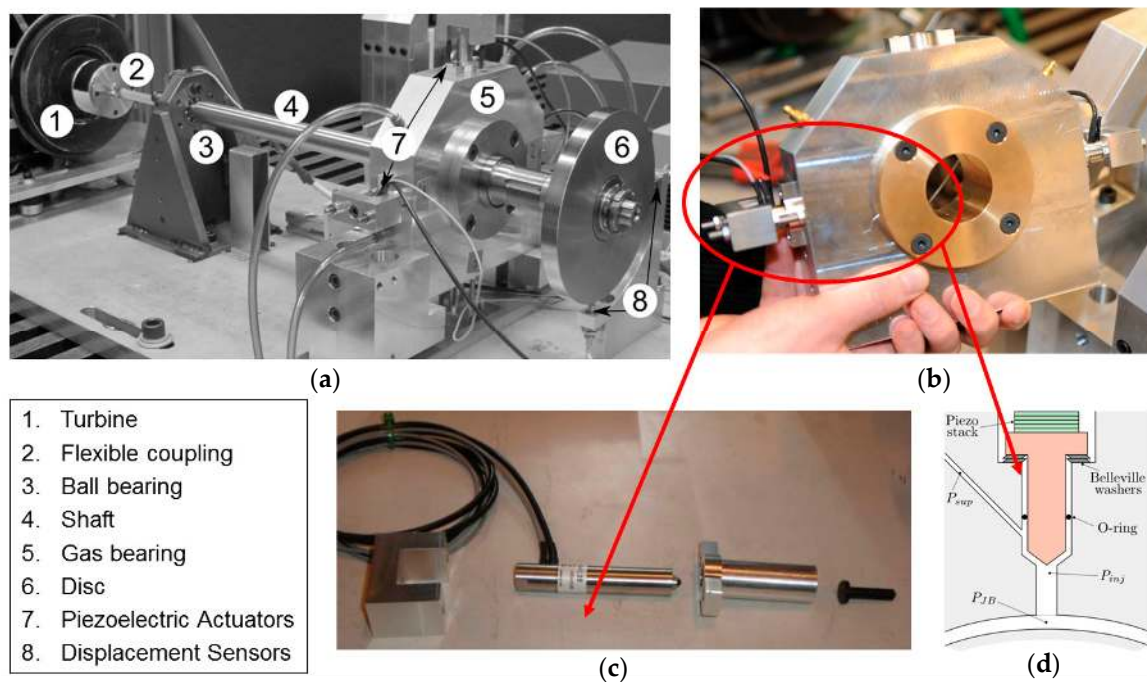
Figure 1. Design details and test bench of controllable radial sliding bearing: (a) the test rig composed of a flexible rotor supported by an actively air lubricated radial bearing, where eddy-current sensors provide information about the rotor lateral vibrations; (b) the piezoelectrically-controlled air lubrication; (c) the piezoelectric actuator; (d) the piezoelectrically-controlled air injection.
