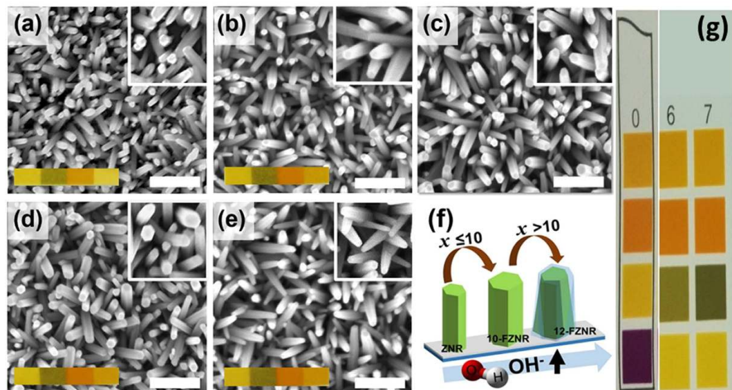
Figure 1. FESEM top-view images of (a) ZNR, (b) 5-FZNR, (c) 8-FZNR, (d) 10-FZNR, (e) 12-FZNR samples, (f) schematic diagram of FZNR growth evolution, and (g) standard litmus pH scale. Scale bar represents 100 nm.
