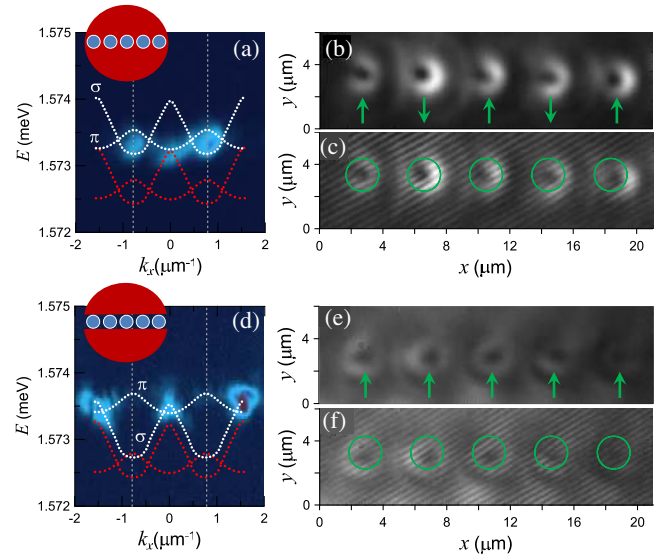
FIG. 2. Photoluminescence above the condensation threshold. (a) Dispersion of exciton polaritons excited by a large-area pump spot (inset, not to scale). Two distinct peaks at the edges of the Brillouin zone (BZ) are visible. The signal in the center of the BZ was detected for k_y \neq 0 . The dotted white lines represent the calculated dispersion subbands, which are blueshifted with respect to the linear dispersion subbands shown by the red dotted lines. (b) The intensity profile of the antiferromagnetic vortex chain measured in real space and (c) the associated interferometry image. (d) Dispersion of exciton polaritons excited by a large-area pump spot with the mesas shielded by a mask (inset, not to scale). (e) The real-space intensity profile of the ferromagnetic vortex chain and (f) the associated interferometry image. The on-site topological charges +1 and -1 are represented by the up and down arrows, respectively. Lack of circular symmetry in (b) and (e) is due to unequal population of the Bloch modes forming the vortex chain (see text).
