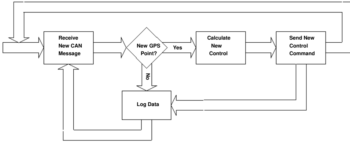
Figure 10. Task computer control program flowchart.
