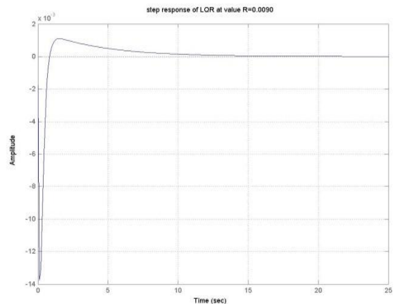
Fig5:- LQR response
