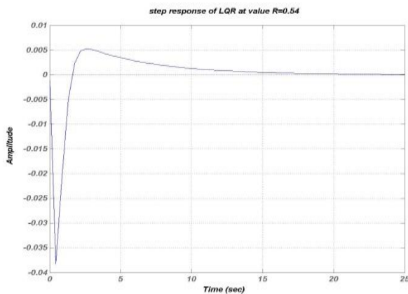
Fig3:- LQR response
