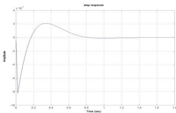
Fig10:- Response of Angle as output using state feedback controller
