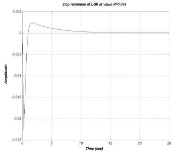
Fig4:- LQR response
