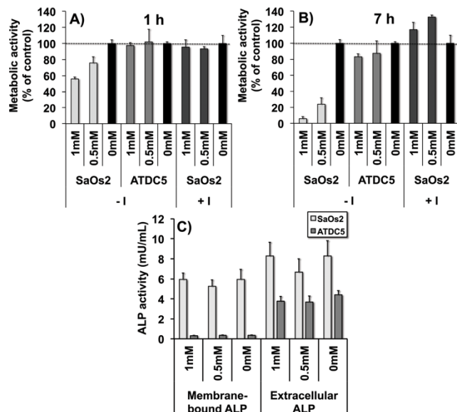
Figure 3. Metabolic activity of SaOs2 and ATDC5 monolayer cultures in the presence of different concentrations of 1 (control – 0 mM, 0.5 mM and 1 mM), without (-) and with (+) phosphatase inhibitor. Values refer to (A) 1 h and (B) 7 h of cell culture. (C) Activity of the membrane bound and extracellular ALP in the
