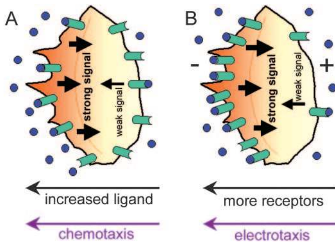
FIG. 18. Model proposed for chemotaxis (A) and electrotaxis (B) of epithelial cells. A: in chemotaxis a gradient of ligand stimulates activation of more receptors on one side of the cell than the other. The result is increased cytoplasmic signaling on one side of the cell relative to the other, even if the receptor density is the same on each side. The side of the cell with higher signaling becomes the leading edge, and the cell migrates up the ligand gradient. B: in electrotaxis, asymmetric signaling results from an increase in density of membrane receptors (or membrane) on the cathode-facing side of the cell. The intracellular signal is higher on the cathode-facing side of the cell, which becomes the leading edge, and the cell migrates toward the cathode.
