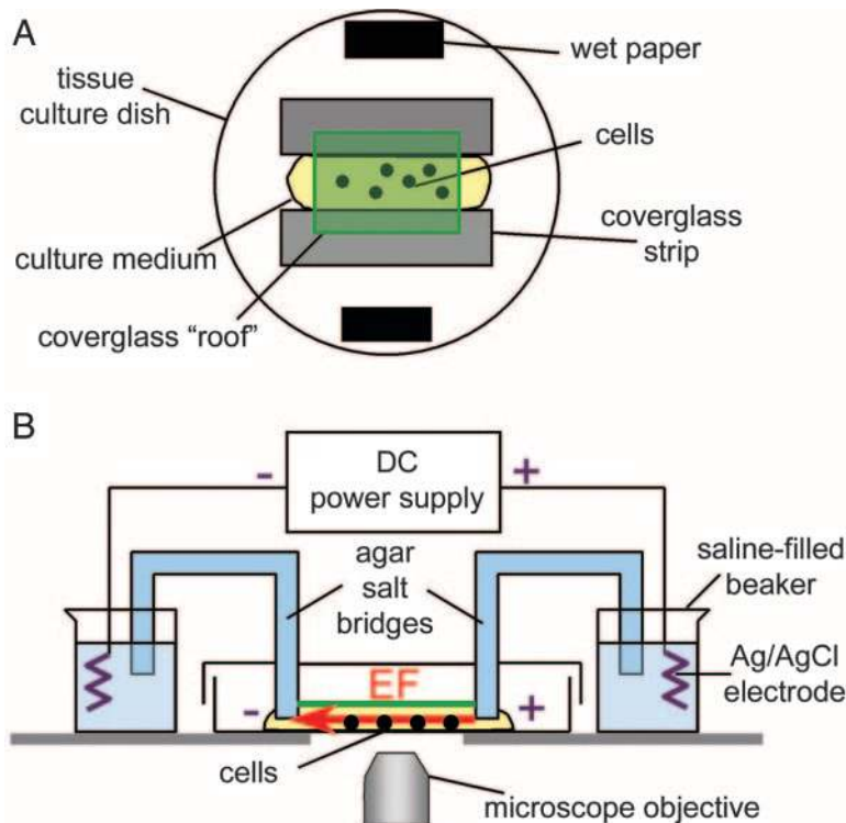
FIG. 14. Method of electric field application. A : top view of chamber. Chambers are made from standard 100-mm tissue-culture dishes. Two strips of number 1 coverglass are secured to the bottom of the dish parallel to each other, 1 cm apart. Cells are plated into the resulting trough, and another coverglass is secured over the top with silicone grease, spanning the entire trough. Strips of paper saturated with water are placed in the dish to maintain humidity. B : side view. Electrical contact is made to the chamber by inserting glass tubes filled with a salt solution gelled with 1% agar through holes in the lid of the chamber. One end of each tube rests in a pool of culture medium continuous with the medium in which the cells are growing; the other end of each tube is placed in a beaker of saline. Ag/AgCl electrodes in each beaker are attached to a direct-current (DC) power supply. Fine adjustments to the EF strength are made via a variable resistor in series with the power supply. Field strength is checked periodically by measuring the voltage drop across the length of the central trough directly using a voltmeter.
