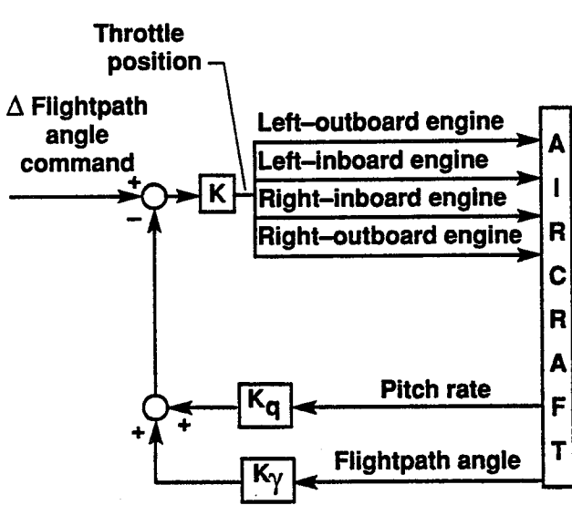
Figure 7. F-15 augmented control block diagram.
