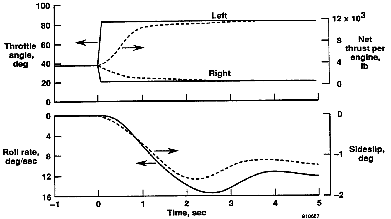
Figure 1. Roll control resulting from differential thrust.
