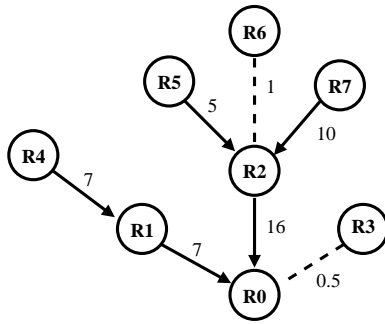
Figure 5: Pushback status messages reporting the aggregate's arrival rate from upstream.
