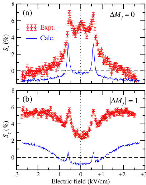
FIG. 2 (color online). Dependence of the measured Ps annihilation signal ( S_\gamma ) on the electric field for photoexcitation with the laser radiation linearly polarized (a) parallel, and (b) perpendicular to the external fields ( B = 13 mT). Experimental data (open circles) and the results of Monte Carlo calculations (continuous curves) are displayed. The calculated values of S_\gamma incorporate only experimental parameters and have not been arbitrarily scaled.
