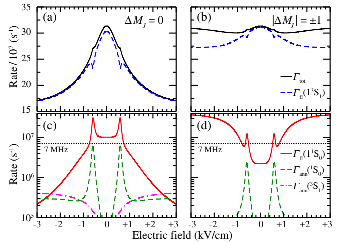
FIG. 3 (color online). Spectral-intensity-weighted average n = 2 decay rates when B = 13 mT for photoexcitation via (a) and (c) \Delta M_J = 0 , and (b) and (d) |\Delta M_J| = 1 transitions from the 1^3S_1 level. (a) and (b), total n = 2 decay rates \Gamma_{\text{tot}} (continuous black curve) and triplet fluorescence rate \Gamma_{\text{fl}}(1^3S_1) (dashed blue curve). (c) and (d), fluorescence rate to the 1^1S_0 level, \Gamma_{\text{fl}}(1^1S_0) , (continuous red curve), and direct 2^1S_0 , \Gamma_{\text{ann}}(1^1S_0) , (dashed green curve) and 2^3S_1 , \Gamma_{\text{ann}}(2^3S_1) , (dash-dotted magenta curve) annihilation rates. The horizontal dashed lines in (c) and (d) correspond to the 7 MHz annihilation rate of the 1^3S_1 state.
