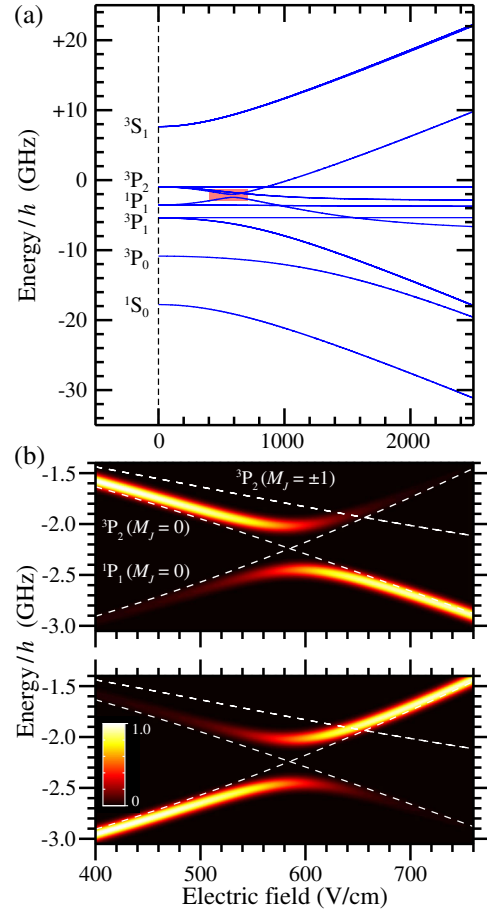
FIG. 1 (color online). (a) Calculated Stark energy level diagram for n = 2 levels of Ps in a parallel magnetic field of B = 13 mT. The energies on the vertical axis are displayed with respect to the n = 2 energy given by the Rydberg formula. The 85 GHz bandwidth of the laser encompasses the entire n = 2 Stark manifold. (b) Expanded view of the region at the avoided crossing between the 2^3P_2 ( M_J = 0 ) and 2^1P_1 ( M_J = 0 ) sublevels highlighted by the shaded red rectangle in (a). The color map in the upper [lower] panel in (b) indicates the 2^3P_2 ( M_J = 0 ) [ 2^1P_1 ( M_J = 0 )] character of each sublevel at the avoided crossing. The dashed lines in each panel indicate the Stark shifts of each sublevel when B = 0 . The color scale in the lower panel is common to both.
