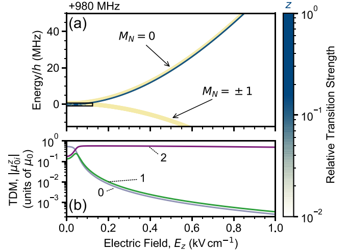
FIG. 2. (a) The energy levels of RbCs ( N=1 ) in a dc electric field and a magnetic field of 181.5 G. The relative transition strengths are shown in Fig. 1(b). (b) The transition dipole moments of the transitions (0, 5)_0 \rightarrow (1, 5)_k for k = 0, 1, 2 [as labeled in Fig. 1(a)] as a function of the electric field.
