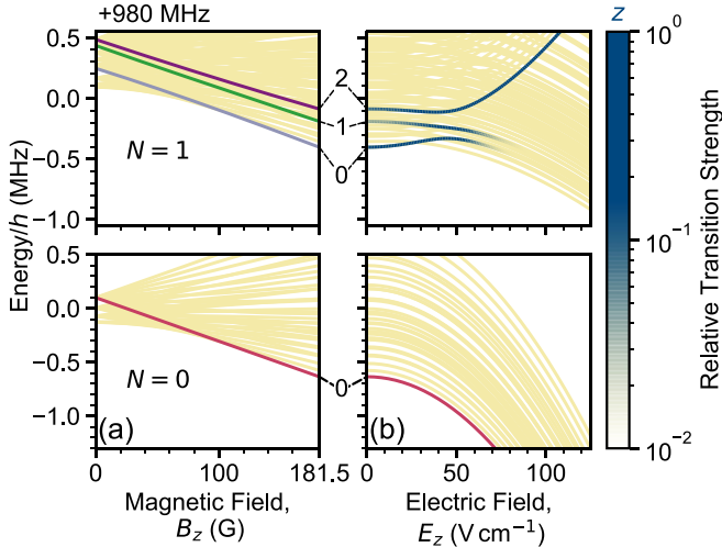
FIG. 1. The hyperfine structure of RbCs. (a) Energy as a function of dc magnetic field. For N=0 , the state (N, M_F)_k = (0, 5)_0 is highlighted in red and labeled as state 0. For N=1 , the states (1, 5)_k are highlighted and labeled with k = 0, 1, 2 . (b) Energy as a function of dc electric field with magnetic field fixed at B_z = 181.5 G. The relative transition strength for transitions from (0, 5)_0 for microwaves polarized along z is shown by the blue color map.
