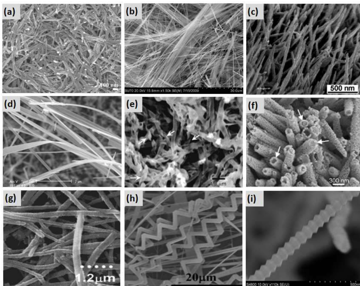
1 2 Fig. 6. SEM images of 1D structures: a) rods ( \gamma -MnO 2 ) (Reprinted with permission. 31 Copyright 2012, 3 Elsevier), b) wires ( \delta -K x V 2 O 5 ) (Reprinted with permission. 32 Copyright 2010, American Chemical 4 Society), c) large arrays of oriented nanotubes (TiO 2 ) (Reprinted with permission. 33 Copyright 2003, 5 American Chemical Society), d) belts (ZnO) (Reprinted with permission. 34 Copyright 2009, 6 Inderscience Enterprises Ltd), e) helical ribbons and the double-layered nanotubes (TiO 2 ) (Reprinted 7 with permission. 35 Copyright 2002, American Chemical Society), f) needles ( \beta -Co(OH) 2 ) (Reprinted 8 with permission. 36 Copyright 2008, John Wiley & Sons), g) hollow fibers (TiO 2 ) (Reprinted with 9 permission. 37 Copyright 2000, American Chemical Society), h) zigzag belts (SnO 2 ) (Reprinted with 10 permission. 38 Copyright 2016, Elsevier), i) zigzag (GaN) (Reprinted with permission. 39 Copyright 2016, 11 Elsevier).
