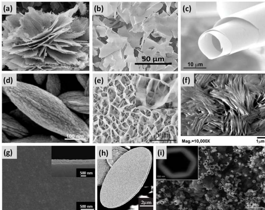
1 2 Fig. 7. SEM images of 2D structures: a) plates (porous ZnO) (Reprinted with permission. 44 Copyright 3 2008, John Wiley & Sons), b) membranes (Fe 2 O 3 ) (Licensed under CC-BY. 45 ), c) membranes 4 (Pd/MnO x /Pd) (Licensed under CC-BY. 46 ), d) mesocrystal disks (Mn 3 O 4 ) (Reprinted with permission. 47 5 Copyright 2014, John Wiley & Sons), e) wall arrays (Ni(OH) 2 ) (Reprinted with permission. 48 Copyright 6 2015, The Royal Chemical Society), f) flakes (ZnO) (Reprinted with permission. 49 Copyright 2013, 7 Elsevier), g) dense film (NiO) (Reprinted with permission. 50 Copyright 2010, Elsevier), h) diskettes 8 (SnO) (Reprinted with permission. 51 Copyright 2003, John Wiley & Sons), i) rings (ZnO) (Reprinted 9 with permission. 52 Copyright 2006, American Chemical Society).
