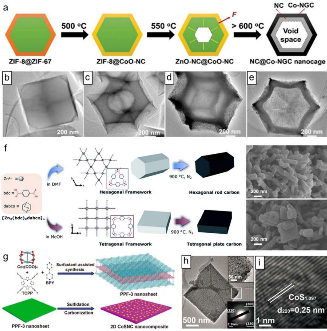
8 9 Fig. 23. Carbon derived from MOF self-templates. a-e) 0D hollow N-doped microporous carbon@Co- 10 N-doped graphitic carbon (NC@Co-NGC) nanocages prepared by external rigid-shell-induced outward 11 contraction (Reproduced with permission. 359 Copyright 2017, John Wiley & Sons). f) Solvent mediated 12 selective synthesis of 1D and 2D MOFs and their transformation to nanoporous carbons (Licensed 13 under CC-BY 360 ). g) Surfactant assisted synthesis of 2D porphyrin paddlewheel framework-3 (PPF-3) 14 nanosheets and their derived CoS/N-doped carbon nanosheets and h, i) the corresponding TEM 15 images of the sample (Reproduced with permission. 361 Copyright 2016, American Chemical Society).
