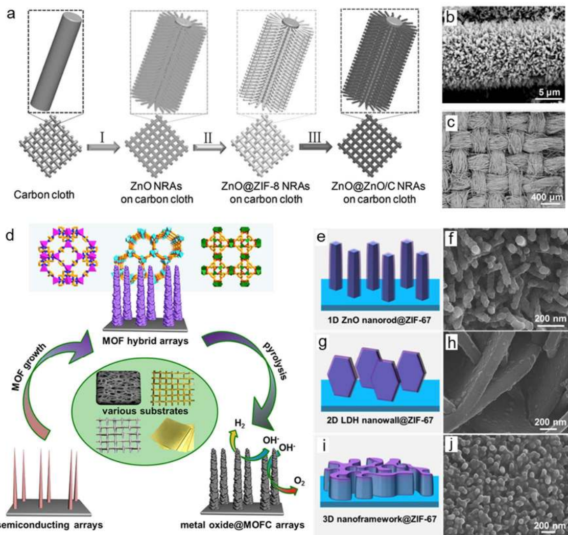
1 2 Fig. 30. 3D carbon array structures. a) Schematic illustrating the synthesis procedures of ZnO@ZnO 3 QDs/C core–shell NRAs on carbon cloth. b, c) High and low magnifications of core–shell ZnO@ZnO 4 QDs/C NRAs grown on flexible carbon cloth (Reproduced with permission. 281 Copyright 2015, John 5 Wiley & Sons). d) Schematic illustration showing the fabrication of MO@MOF hybrid arrays and their 6 derived MO@MOFC arrays on the 3D conductive matrix (Reprinted with permission. 310 Copyright 7 2017, Elsevier). Electrosynthesis of ZIF-67 on Ni-foam supported e, f) 1D ZnO nanorod, g, h) 2D LDH 8 nanowall, and i, j) CoNi-alloy (Reproduced with permission. 428 ).
