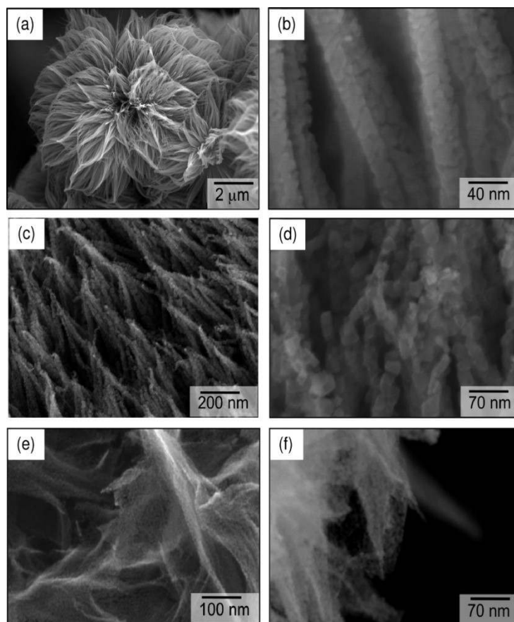
Fig. 11. SEM micrographs of flower-like \text{Co}_3\text{O}_4 nanostructures achieved at 90\text{ }^\circ\text{C} using \text{Co}(\text{NO}_3)_2 \cdot 6\text{H}_2\text{O} as cobalt source: a, b ) necklace and c, d ) net, e, f ) \text{Co}_3\text{O}_4 nanostructures obtained from \text{CoCl}_2 \cdot 6\text{H}_2\text{O} precursor at 70\text{ }^\circ\text{C} and 50\text{ }^\circ\text{C} , respectively (Reprinted with permission. 131 Copyright 2011, American Chemical Society).
