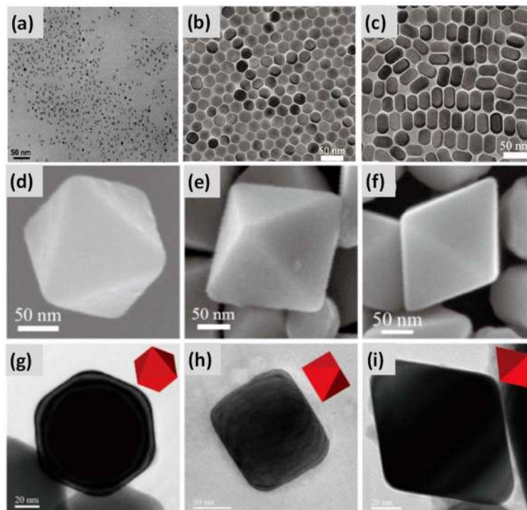
Fig. 5. TEM (a-c, g-i) and SEM (d-f) images of 0D nanostructures: a) quantum dots (CdSe/ZnS) (Reprinted with permission. 24 Copyright 2013, Inderscience), b) spherical nanoparticles ( Mn_3O_4 ), c)
