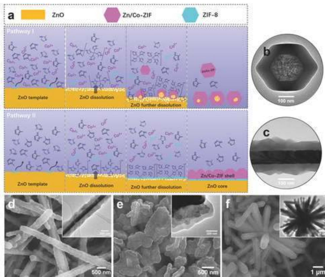
1 2 Fig. 29. Dimension controlled ZnO directed synthesis of hollow carbons. a) Schematic representation 3 of the growth of bimetallic Zn/Co-ZIF using ZnONW as a template under different precursor addition 4 sequences. TEM images of b) ZnO@Zn/Co-ZIF nanopolyhedron and c) core-shell ZnONW@ZIF- 5 8@Zn/Co-ZIF. SEM images and the corresponding TEM images (inset) of d) 1D ZnONW@ZIF- 6 8@Zn/Co-ZIF, e) 2D ZnONP@ZIF-8@Zn/Co-ZIF, and f) 3D ZnONF@ZIF-8@Zn/Co-ZIF. The products 7 were collected at a reaction temperature of 45 °C after 2 h reaction (Reprinted with permission. 426 8 Copyright 2018, John Wiley & Sons).
