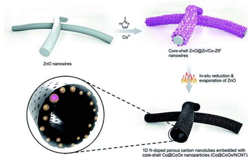
16 17 Fig. 27. 1D ZnO nanowires directed synthesis of Co@CoO x /NCNTs. The magnified view indicates the 18 existence of core–shell Co@CoO x nanoparticles embedded in the porous carbon nanotube (Reprinted 19 with permission. 419 Copyright 2017, The Royal Society of Chemistry).
