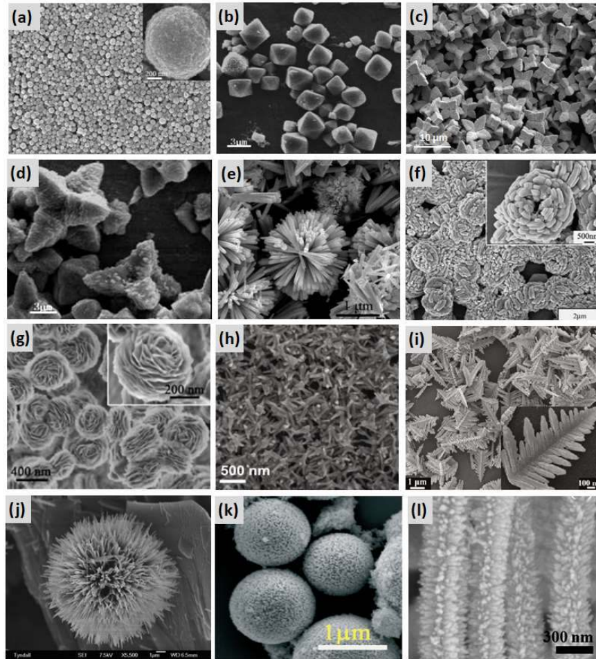
11 12 Fig. 8. SEM images of 3D structures: a) colloidal spheres ( \text{Mn}_3\text{O}_4 ) (Reprinted with permission. 25 13 Copyright 2010, American Chemical Society), b) octahedra ( \text{Cu}_2\text{O} ), c) eightpod cubes ( \text{Cu}_2\text{O} ), d) 14 six-armed starlike \text{Cu}_2\text{O} (Reprinted with permission. 55 Copyright 2009, American Chemical Society), e) 15 \text{ZnO} microsphere consisting of nanorods (Reprinted with permission. 56 Copyright 2009, American 16 Chemical Society), f) doughnut-shaped microparticles ( \text{ZnO} ) (Reprinted with permission. 57 Copyright 17 2005, American Chemical Society), g) flowers ( \beta\text{-Ni(OH)}_2 ) (Reprinted with permission. 58 Copyright 18 2014, The Royal Chemical Society), h) multipods ( \text{Ni} ) (Reprinted with permission. 54 Copyright 2018, 19 American Chemical Society), i) dendritic structures ( \gamma\text{-Fe}_2\text{O}_3 ) (Reprinted with permission. 59 Copyright 20 2011, American Chemical Society), j) urchin ( \text{VO}_x ) (Reprinted with permission. 60 Copyright 2006, 21 American Chemical Society), k) balls ( \text{Mn}_2\text{O}_3 ) (Reprinted with permission. 61 Copyright 2016, The Royal 22 Chemical Society), l) branches ( \text{TiO}_2\text{-SnO}_2 ) (Reprinted with permission. 62 Copyright 2013, The Royal 23 Chemical Society).
