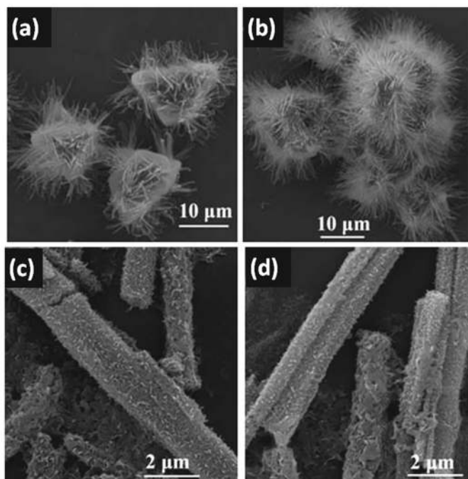
Fig. 16. SEM images of urchin-like CuO superstructures prepared by immersing octahedral Cu-MOFs in 0.1M NaOH at room temperature for a) 5 h or b) 12 h and SEM images of rod-like CuO superstructures obtained by immersing six-prismatic Cu-MOFs in 0.1M NaOH for c) 30 min or d) 5 h (Licensed under CC-BY. 224 ).
