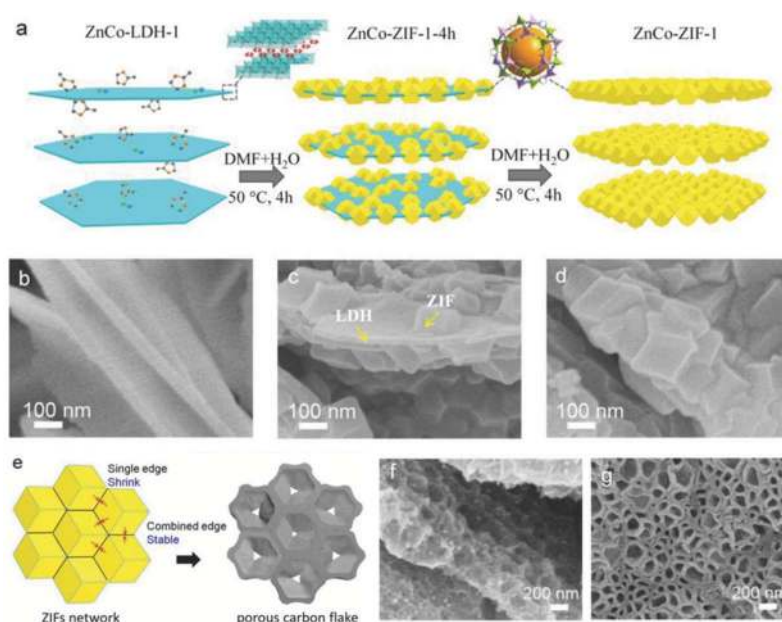
1 2 Fig. 28. 2D ZnCo-LDH derived synthesis of 2D ZIF and carbon flakes. a) Schematic illustration of the 3 synthesis of ZIF networks. SEM images of b) ZnCo-LDH-1, c) ZnCo-ZIF-1-4h, and d) ZnCo-ZIF-1. e) 4 Schematic illustration of the pore formation mechanism. SEM images of f, g) 2D honeycomb-like 5 carbon flakes (Reproduced with permission. 423 Copyright 2018, John Wiley & Sons).
