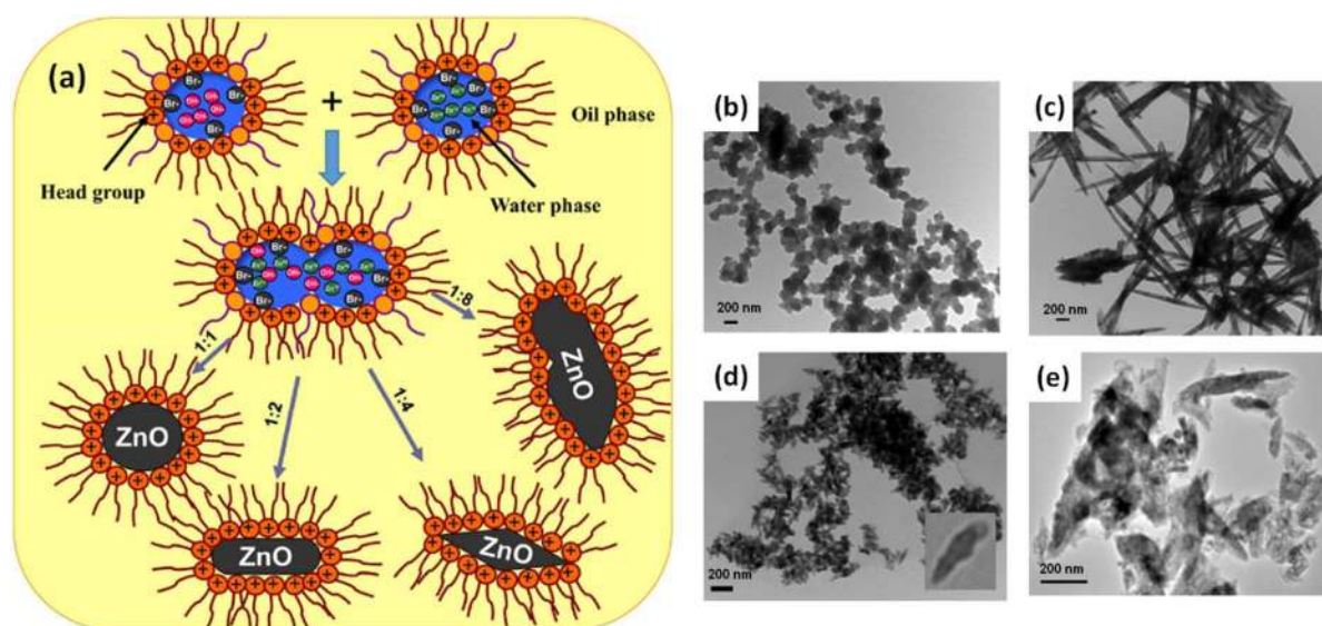
Fig. 13. a) Zn 2+ , Br - , and OH - ion interaction and effect of [Zn 2+ ]:[OH - ] ratio on ZnO nanoparticle morphologies. TEM images of ZnO with b) spherical, c) needle-like, d) acicular, and e) irregular shapes (Licensed under CC-BY. 163 ).
