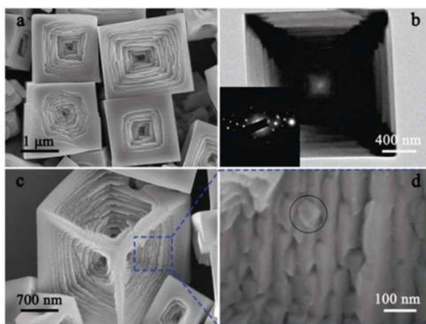
17 18 Fig. 33. a) FESEM image of the sample prepared following a typical procedure. b) TEM and c, d) high 19 magnification FESEM images of a single hierarchical PW crystals. Inset: selected area electron 20 diffraction (SAED) pattern taken from the edge section. (Reprinted with permission. 501 Copyright 21 2014, The Royal Chemical Society).
