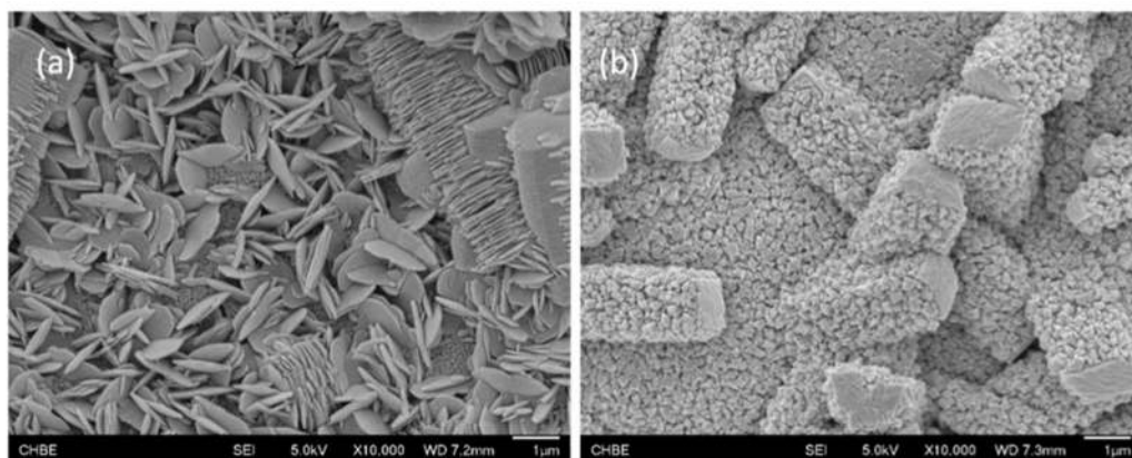
1 2 Fig. 32. Flower-like (left) and ordered nanocrystals (right) morphology of NH 2 -MIL-53(Al) of the 3 second growth tubes for seawater desalination (Licensed under CC-BY. 482 ).
