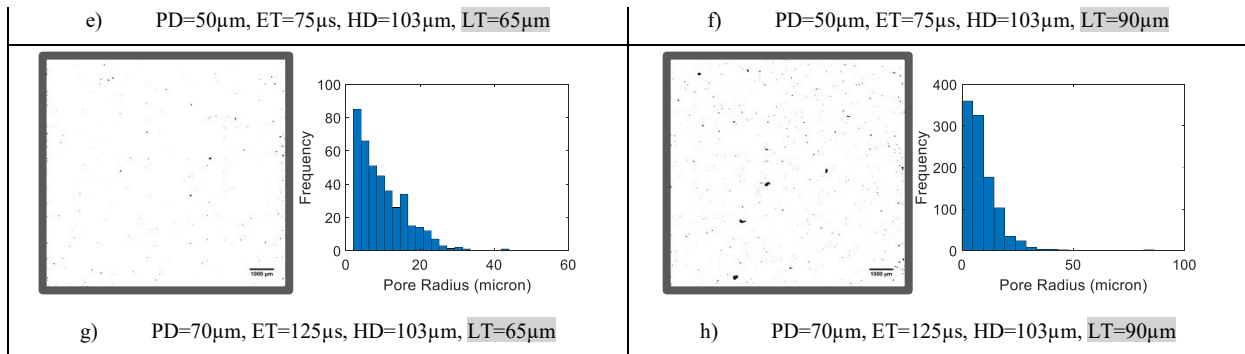
Figure 8: Optical micrographs and Histogram analysis showing the effects of LT on the amount and size of pores. All the scale bars are 1000μm.
