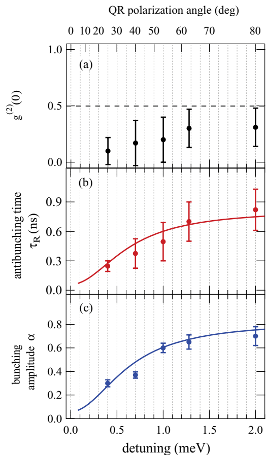
FIG. 3. (Color online) Extracted values of (a) g^2(0) , (b) antibunching time \tau_R , and (c) bunching amplitude \alpha vs detuning from the results of Fig. 2. The black dashed line in (a) indicates the SPE limit, while the solid lines in (b) and (c) are fits with Eqs. (5) and (6), respectively.
