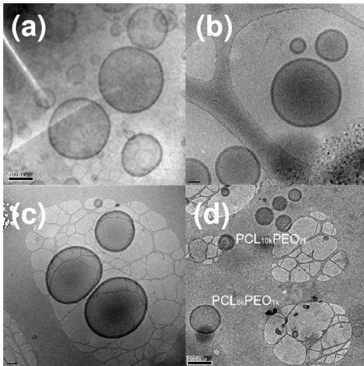
Figure 9: Cryo-TEM images of the vesicles in 28 % THF in water. Panels a and b show the vesicles obtained from the self-assembly of \text{PCL}_{5\text{k}}\text{PEO}_{1\text{k}} and \text{PCL}_{10\text{k}}\text{PEO}_{2\text{k}} , respectively. Panel c shows the structures obtained when solutions of \text{PCL}_{5\text{k}}\text{PEO}_{1\text{k}} and \text{PCL}_{10\text{k}}\text{PEO}_{2\text{k}} in pure THF are mixed in equal parts prior to self-assembly. Panel d shows the same composition when the two solutions are mixed after self-assembly at a THF content of 28%. The image was taken 1 week after mixing. Two distinct populations of vesicles with different wall thickness can be seen. All images are at the same magnification. The scalebars in a and d are 200 nm and 100 nm in panels b and c.
