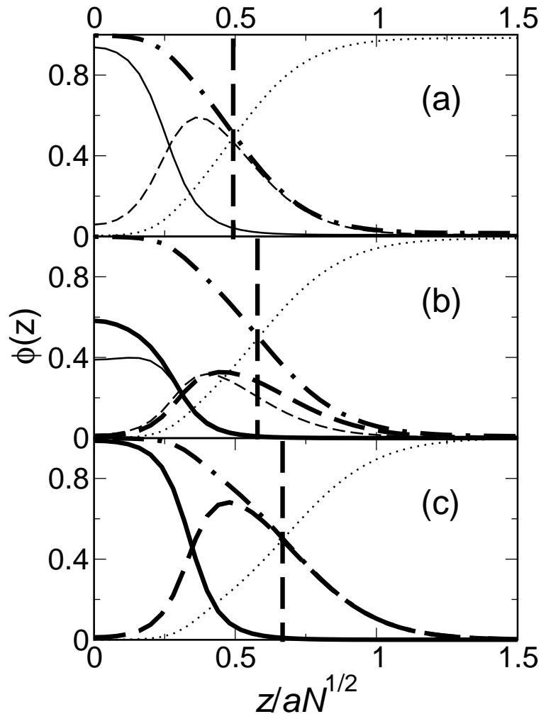
Figure 10: Density profiles of an infinite lamellar structure in (a) an N/2 -monomer lamella-former, (b) a 1:1 blend of 3N/4 -monomer lamella-former and N/2 -monomer lamella-former and (c) a 3N/4 -monomer lamella-former. The hydrophobic and hydrophilic block density profiles are shown with full and dashed lines respectively, and the 3N/4 lamella-formers are plotted with thicker lines. The solvent is plotted with a dotted line, the total density of copolymers is plotted with a dot-dashed line, and the point at which these two densities are equal is marked with a thick vertical dashed line.
