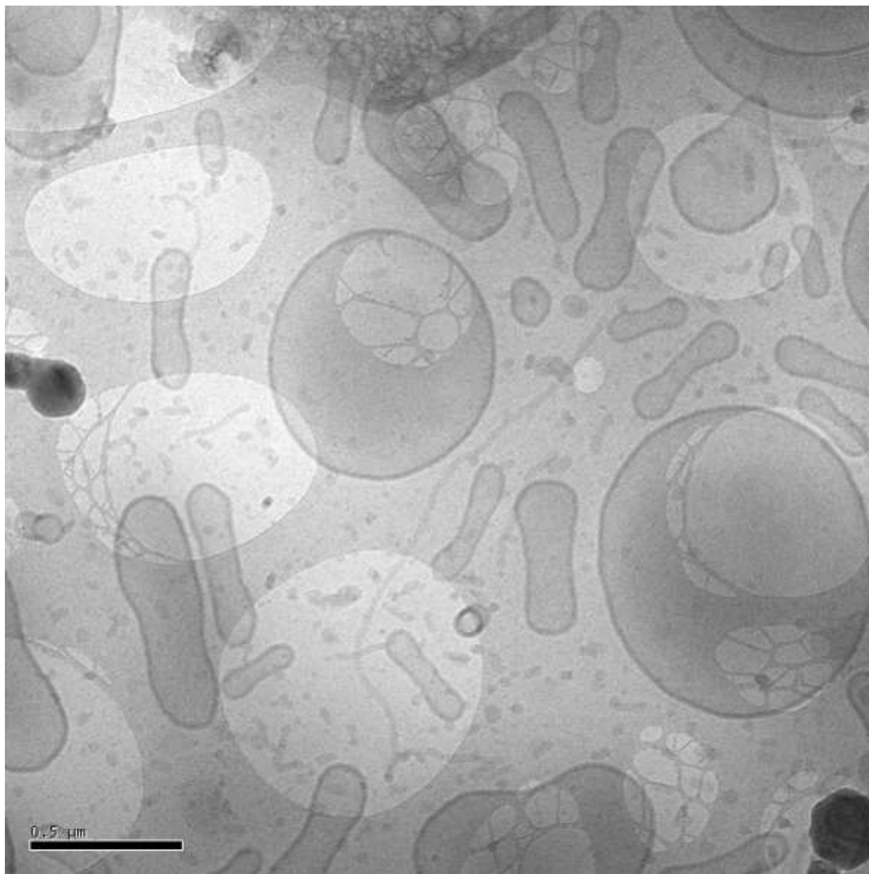
Figure 11: Cryo-TEM of the self-assembled structures obtained for a mixture of PCL 5k PEO 550 and PCL 5k PEO 2k at a mass-based mixing ratio of 3 to 2 parts. The image was taken from a solution containing 28% THF and the scalebar is 500 nm.
