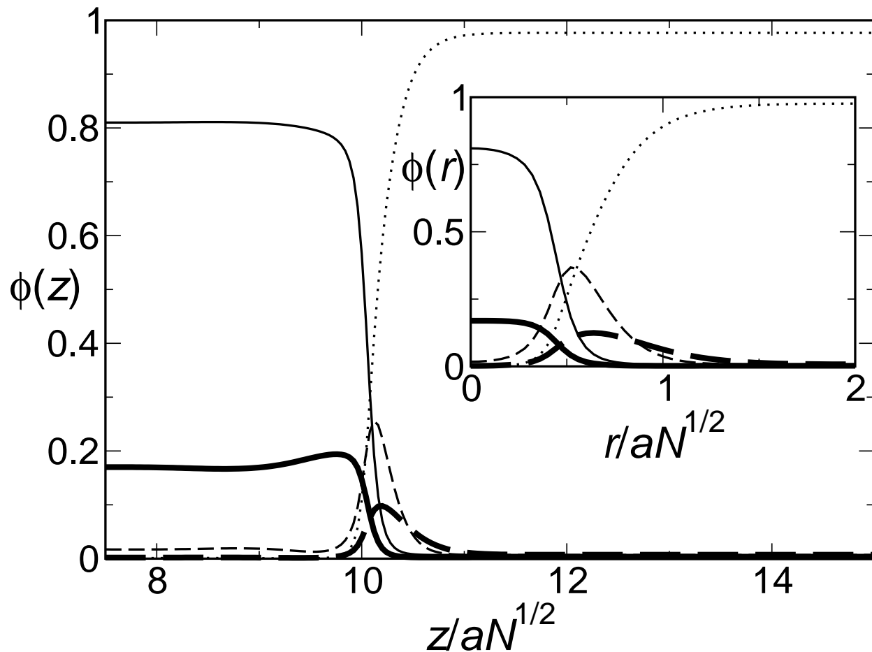
Figure 7: Cuts through the density profiles of the rod structure in a 2:1 blend of N/2 -monomer lamella-former and N -monomer sphere-former. The hydrophobic and hydrophilic block density profiles are shown with full and dashed lines respectively, and the sphere-formers are plotted with thicker lines. The solvent is plotted with a dotted line. The main panel shows a cut along the main axis of the rod and the inset shows a cut perpendicular to this axis at the center of the rod.
