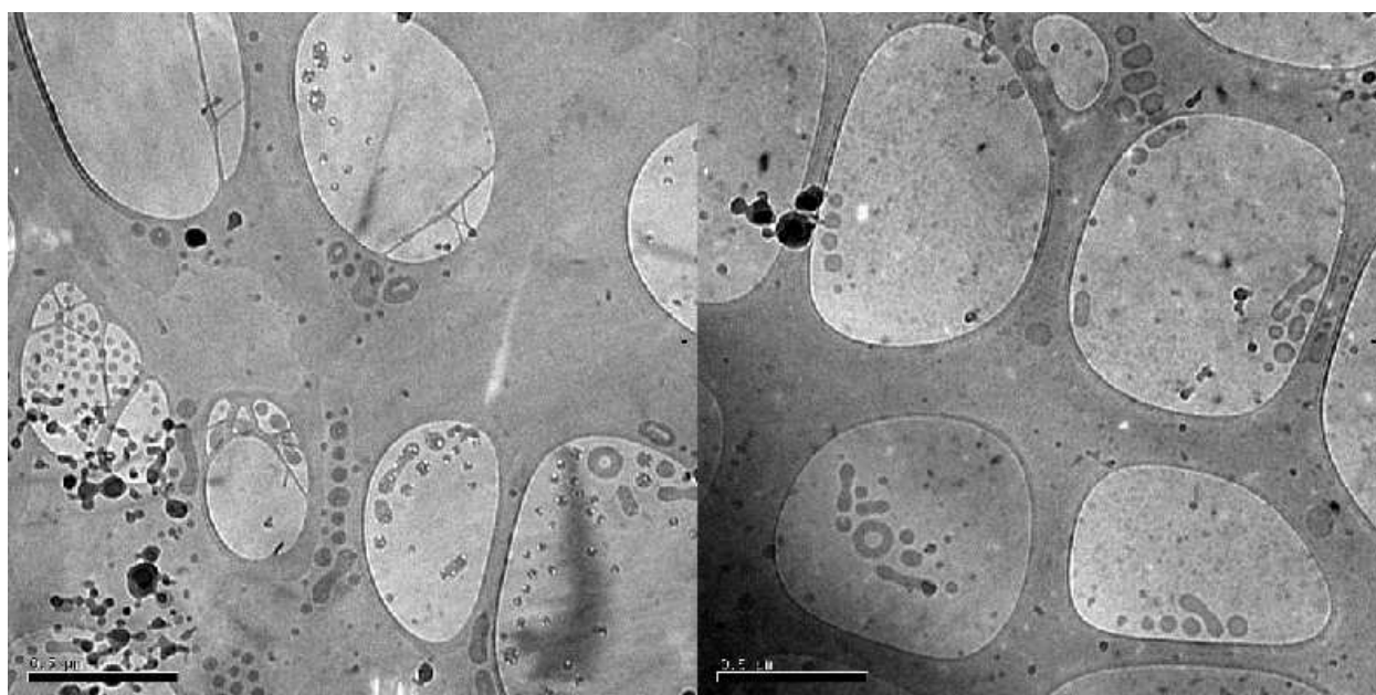
Figure 3: Cryo-TEM of a mixture of 80% PCL 10k PEO 2k and 20% PCL 5k PEO 2k self-assembled by solvent exchange from THF. The images were taken in an aqueous solution with 28% THF; the scalebars are 500 nm.
