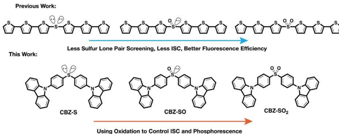
Fig. 2 Design principle and chemical structures of sulfur-bridged dimers for fluorescent and phosphorescent materials.
