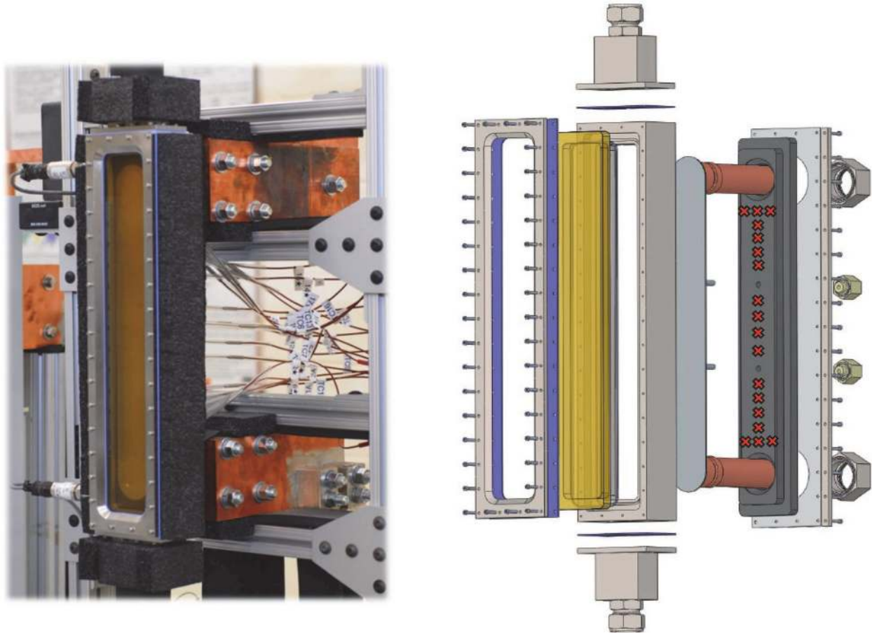
Fig. 3 The narrow rectangular coolant channel test section. The channel is heated on one side, with a polysulfone viewing window on the front face. Thermocouple locations are indicated by X's in the CAD model on the right.
