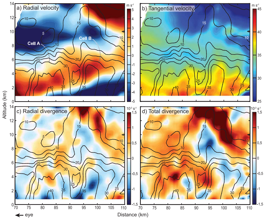
FIG. 17. Averaged vertical cross section of (a) radial velocity, (b) tangential velocity, (c) radial divergence, and (d) total divergence from outlined section in Fig. 16. Reflectivity values are overlaid as black contours (dBZ). Cells A and B are indicated.
