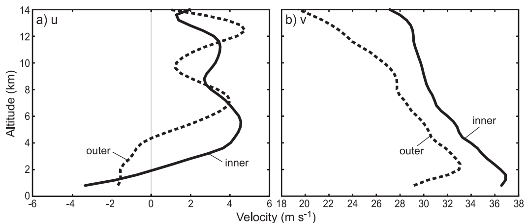
FIG. 7. Vertical profiles of the (a) mean radial and (b) mean tangential velocity for pixels classified as convective in the inner and outer upwind regions.
