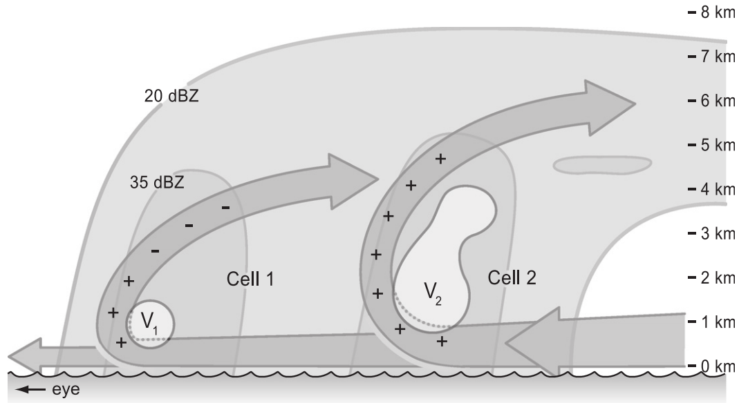
FIG. 18. Schematic of the convective motions associated with two mature convective cells at different radial distances from the storm center within the inner core. Reflectivity contours are drawn showing cell 1 at a smaller radius and cell 2 at a larger radius. The solid arrows represent the overturning secondary circulation within each cell, and the plus (minus) signs indicate regions of increasing (decreasing) tangential velocity; V_1 and V_2 represent the tangential velocity jets in each cell.
