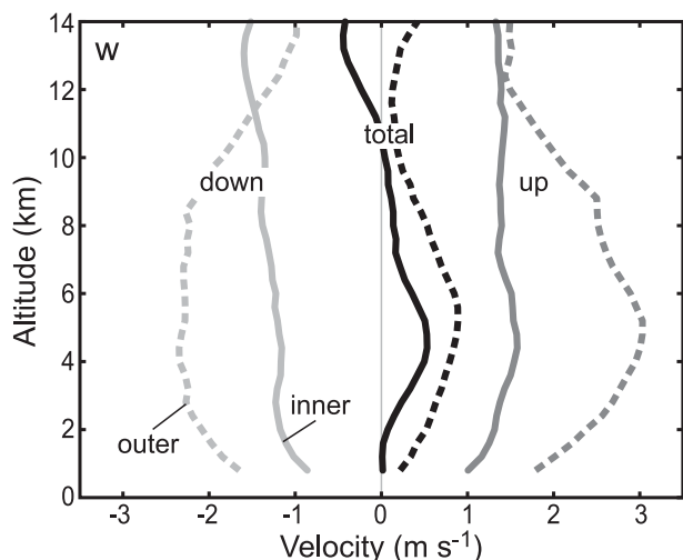
FIG. 6. Vertical profiles of the mean vertical velocity for pixels classified as convective in the upwind inner region (solid) and the upwind outer region (dashed). Profiles displayed are updrafts, downdrafts, and total vertical velocity.
