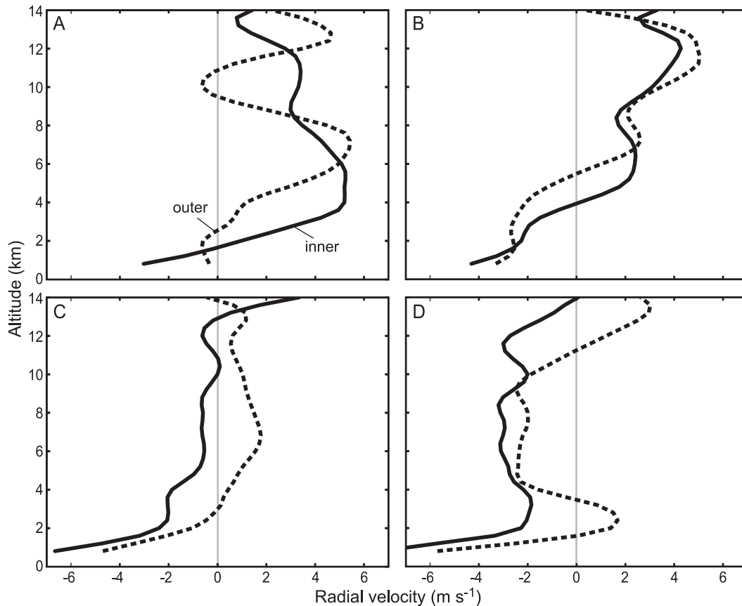
FIG. 14. Vertical profiles of the mean radial velocity in the inner and outer regions for sections A–D.
