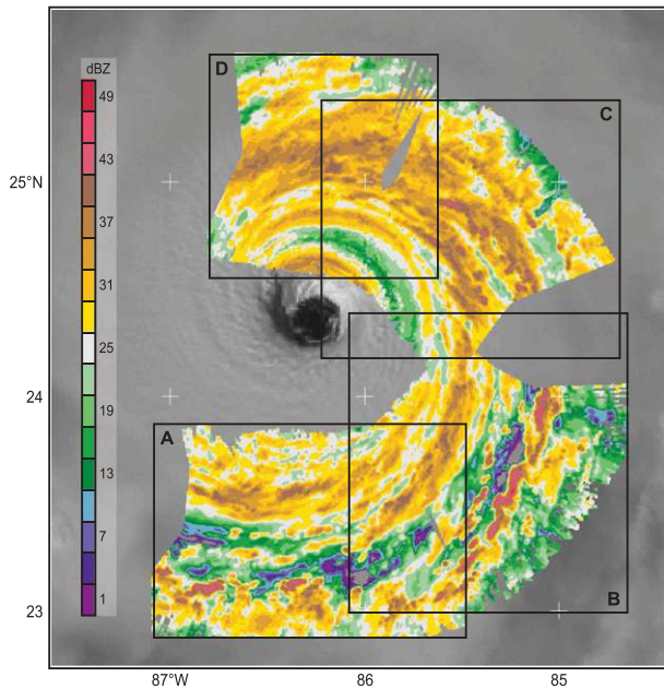
FIG. 1. Plan view of ELDORA reflectivity data at 2-km altitude observed during 1845–1927 UTC 21 Sep 2005. Visible imagery from Geostationary Operational Environmental Satellite-East is shown in the background. Boxes outline sections A–D used in the analysis.
