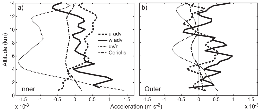
FIG. 11. As in Fig. 8, but for tangential momentum budget terms from Eq. (4).
