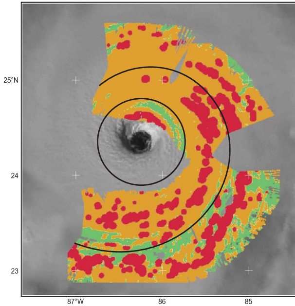
FIG. 2. Results of convective–stratiform separation algorithm applied to ELDORA reflectivity data shown in Fig. 1. Red indicates convective regions, orange indicates stratiform regions, and green indicates weak-echo regions. The overlying black circle encompasses the eyewall convection and the black spiral divides the inner convection from the outer convection.
