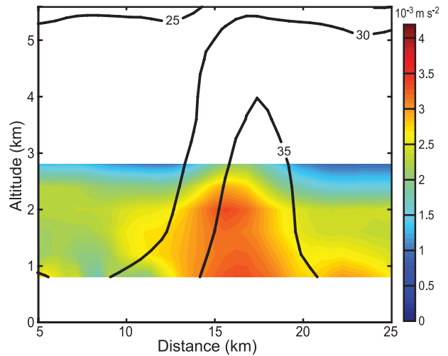
FIG. 10. Composite of GBR values from radially aligned cross sections of convective cells in the inner upwind region: average reflectivity values are overlaid as black contours (dBZ).
