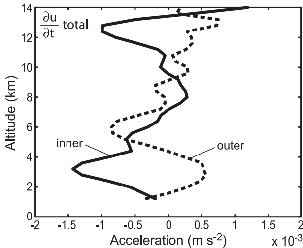
FIG. 9. Summed vertical profiles of the mean radial momentum budget terms from the convective pixels in the upwind inner and outer regions.
