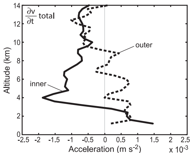
FIG. 12. As in Fig. 9, but for tangential momentum budget terms.
