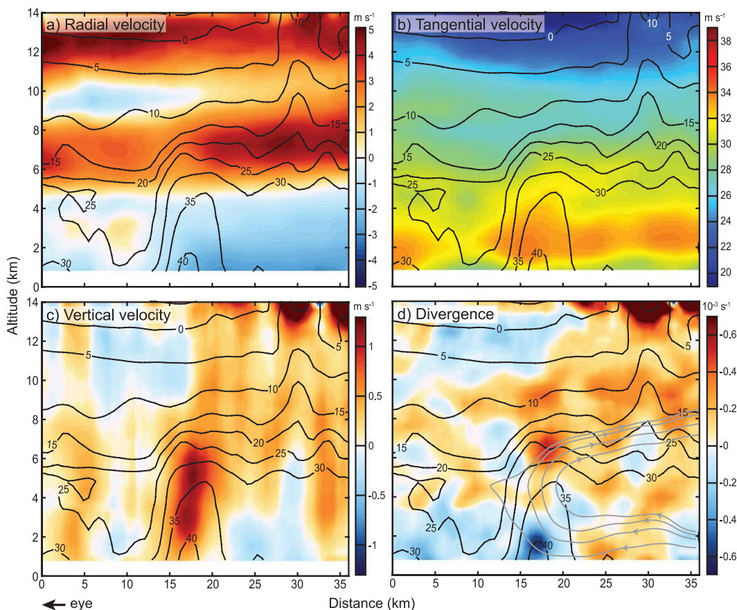
FIG. 4. As in Fig. 3, but for cross sections of convective cells in the outer upwind region.
