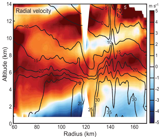
FIG. 13. Azimuthally averaged field of radial velocity from sections A and B; average reflectivity values are overlaid as black contours (dBZ).
