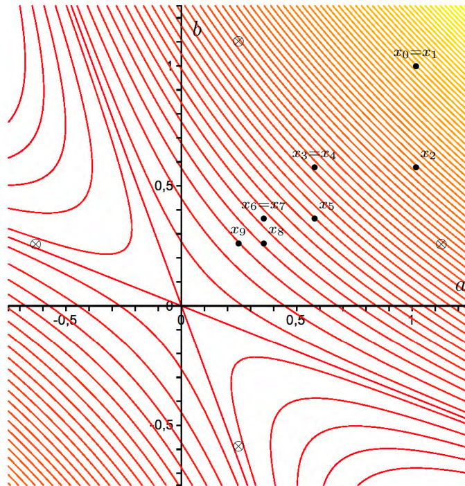
Figure 1: Initial iterates of GPS
