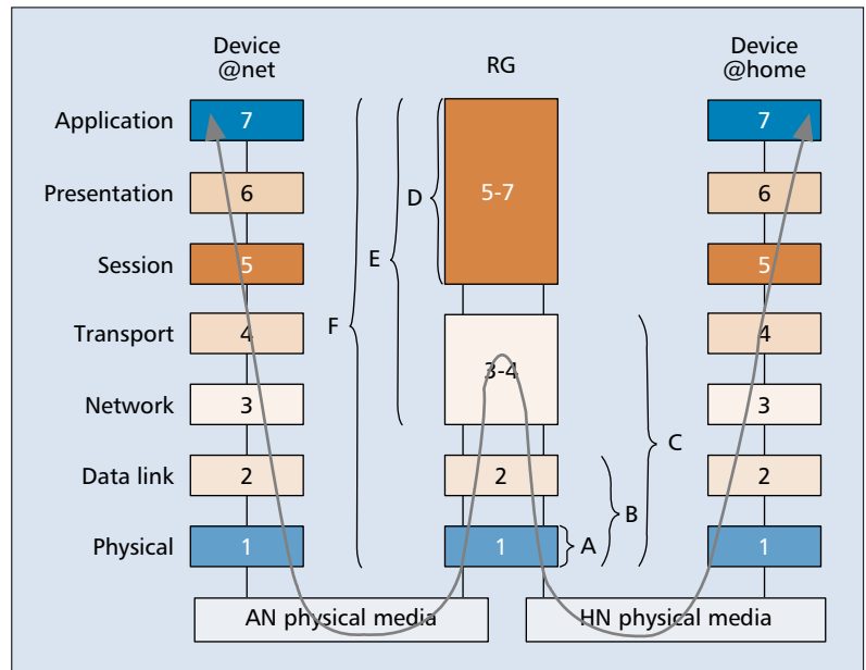
■ Figure 1. RG classification model based on OSI.
