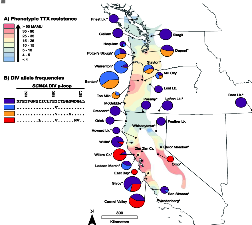
Figure 2. A) Average phenotypic TTX resistance (50% MAMU) in populations of Th. sirtalis in western North America. Estimates are interpolated across the geographic range wherein Th. sirtalis occur in sympatry with Taricha newts (recreated from Brodie et al. 2002). B) Pie charts indicate observed population frequencies of the four unique DIV alleles identified in this study. Chart size is proportional to the sample size at each location. All localities used in the phylogenetic analysis are marked with an asterisk (*).
