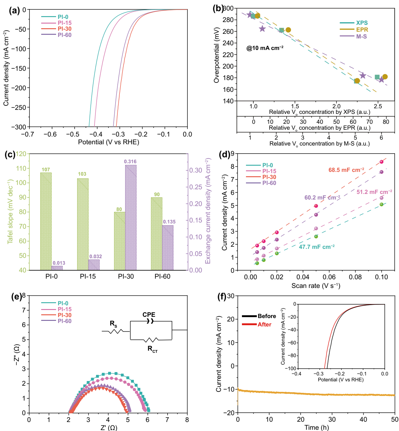
Fig. 5 Electrocatalysis performance of 2D \text{Bi}_2\text{O}_3 nanosheets in 1.0 M KOH. Polarization curves collected at a scan rate of 5 \text{ mV s}^{-1} (a). The relationship of the overpotentials needed to reach j=10 \text{ mA cm}^{-2} and the relative oxygen vacancy concentrations obtained from EPR, XPS and EPR measurements (b). Tafel slopes and exchange current densities for 2D \text{Bi}_2\text{O}_3 nanosheets with different oxygen vacancy concentrations (c). Calculated C_{dl} plots of 2D \text{Bi}_2\text{O}_3 nanosheets at 10 \text{ mA cm}^{-2} (d). EIS measurements on different 2D \text{Bi}_2\text{O}_3 nanosheets. (e) Stability test on the PI-30 up to 50 h (f)
