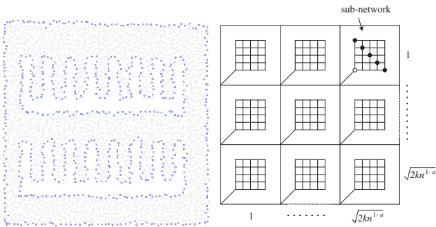
Fig. 2. A network with 3996 nodes, avg degree 9.7.
