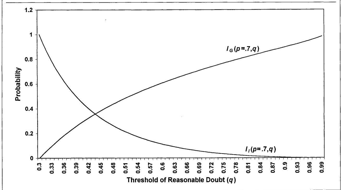
FIGURE 3. Limit Error Probabilities as a Function of the Threshold of Reasonable Doubt
