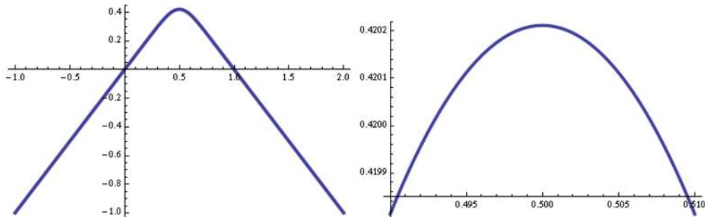
Figure 7: Plot of g using f_c = 0.25 . Right: zoom near the point x = 0.5 .
