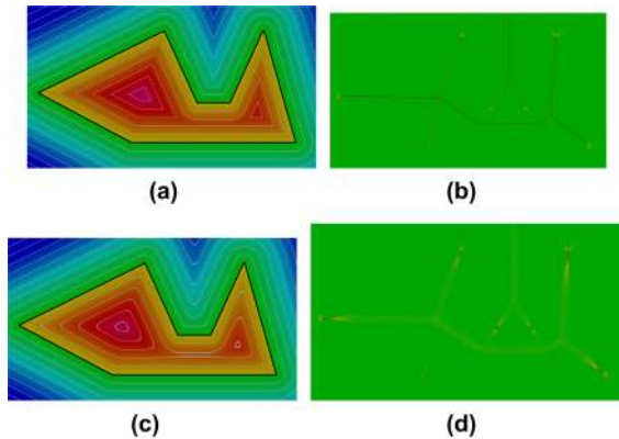
Figure 13: The pictures (a) and (c) show the iso-values of a scalar field, (a) for the signed distance, (c) our method. The pictures (b) and (d) show the derivative discontinuities using edge detection.
