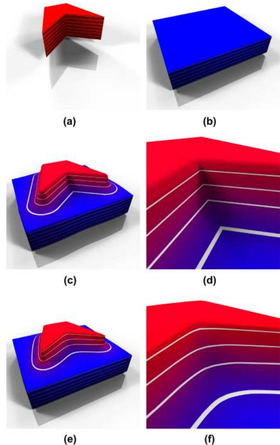
Figure 16: Blending union operation: (a) and (b) show two initial objects; (c) the blending union with signed distances; (d) zoom to the discontinuity area; (e) and (f) show the same operation with filtered signed distances.
