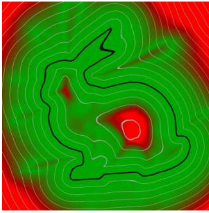
Figure 12: Medial axis detection using the initial samples. Green indicates low sampling rate while red means high sampling rate.
