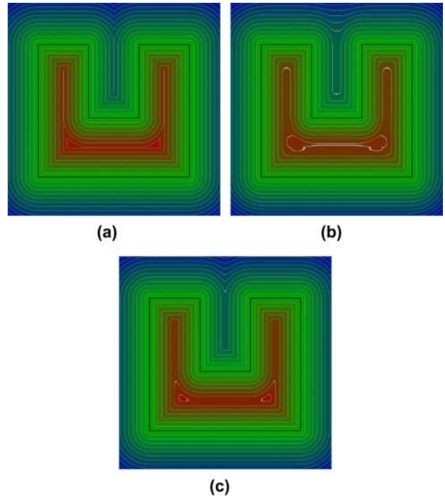
Figure 10: Filtering the distance field: (a) shows the signed distance field, (b) uses a regular grid of samples used with (9), (c) uses (10) with a Gaussian distribution for w and the samples drawn from this distribution.
