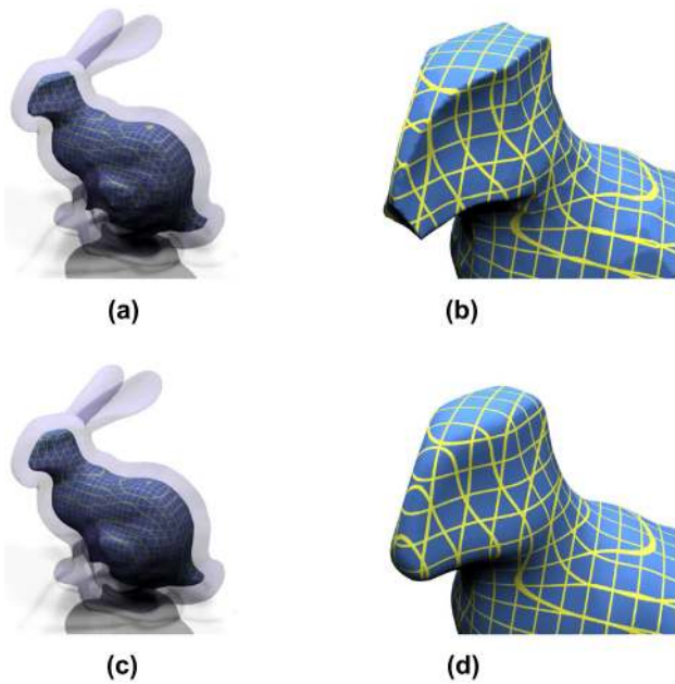
Figure 1: Offset of the Stanford bunny, (a) and (b) using signed distances, (c) and (d) using our method.
