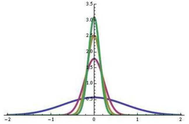
Figure 3: Gaussian weight function for different values of the parameter a : 1 (blue), 10 (purple), 20 (yellow) and 30 (green).
