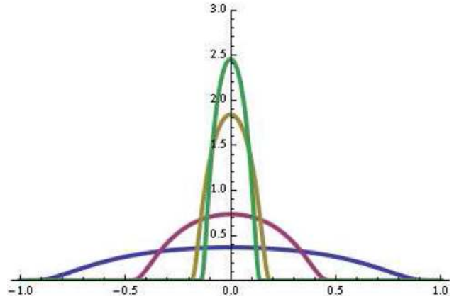
Figure 4: Bump function for various values of the parameter b : 0.15 (green), 0.2 (yellow), 0.5 (purple) and 1 (blue).
