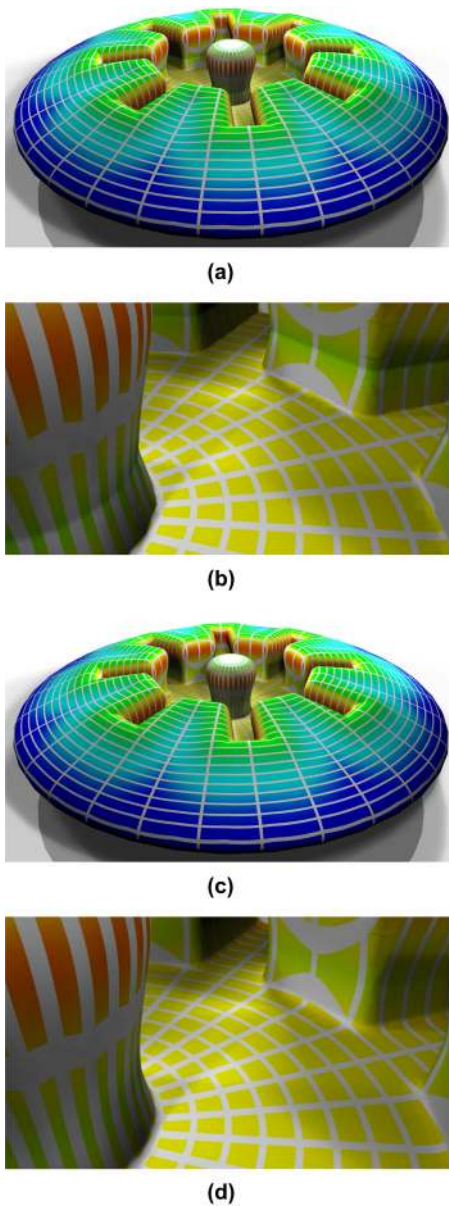
Figure 17: Blending difference operation: (a) the blending difference between a gear and a sphere with signed distances; (b) zoom to the discontinuity area; (c) and (d) show the same operation with filtered signed distances.
