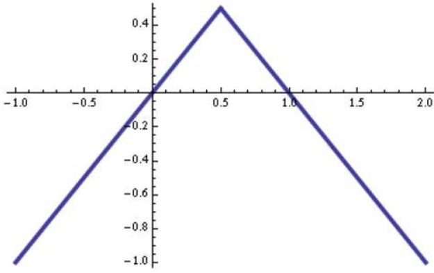
Figure 5: Plot of the distance to the boundary of the segment [0, 1] .
