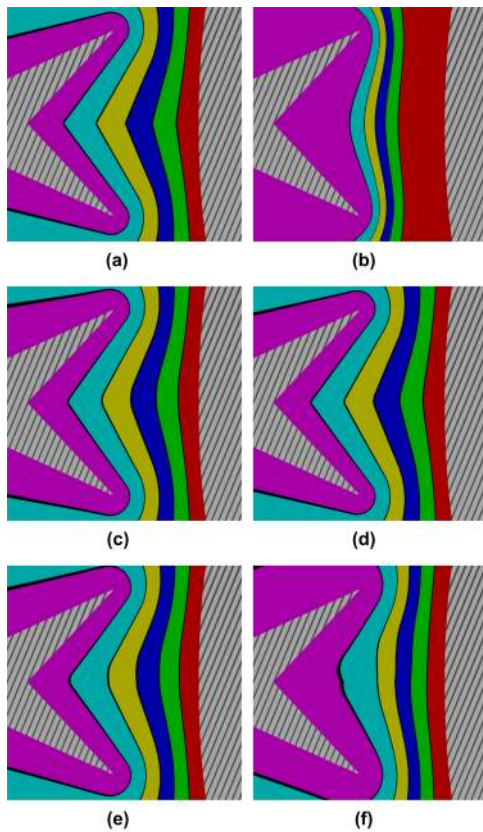
Figure 19: Transfinite interpolation of material properties between two material features: the top left is the distribution of materials using exact signed distances, top right (b) uses the L_1 -dist field. The other examples use filters with various parameters to control the smoothing.
