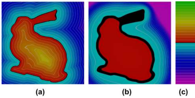
Figure 2: (a) The signed distance field to the Stanford bunny; (b) An approximation of the distance field with the L_p distance field for p = 1 ; (c) The colour-map used in (a) and (b). The black line corresponds to values close to the zero-set (narrow range of zero).
