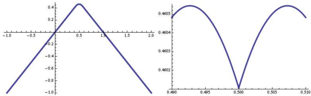
Figure 6: Plot of g using f_c = 1.0 . Right: zoom near the point x = 0.5 .
