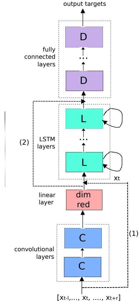
Fig. 1. CLDNN Architecture
