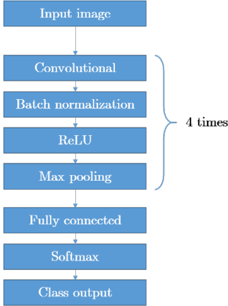
Figure 1. Diagram of the proposed deep learning network in which each box represents a different layer. The input image is a RGB r \times s patch. Visual data is then processed by four deep learning blocks of layers. Finally, a classical neural network followed by a softmax and a class output gives the classification result.
