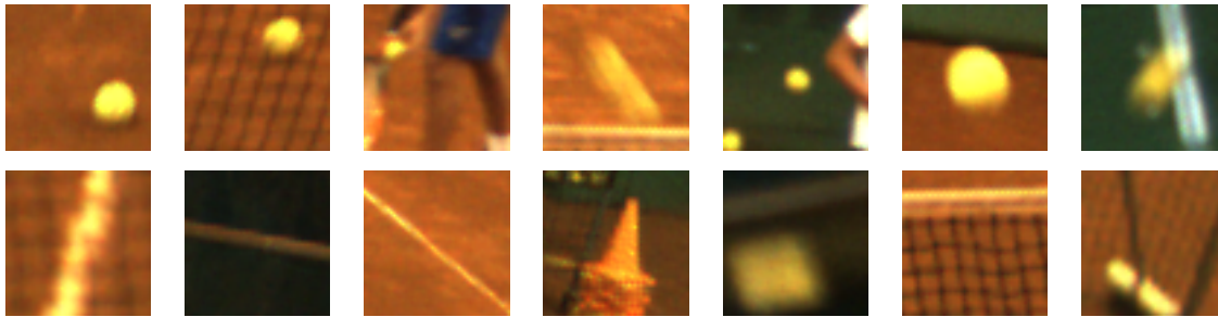
Figure 3. Examples of Ball images (first row) and No Ball images (second row) extracted from the dataset considered in this paper. An image patch has been labeled as Ball without imposing constraints about the position and the size of the ball and including blurred moving balls. The other class is made of examples that are likely to be confused with a ball, such as the court lines (that in image patches can be easily misclassified as a fast moving ball), as well as other sport equipments usually present during training sessions.
