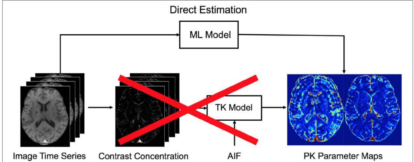
FIGURE 2 | The conventional pipeline of pharmacokinetic parameters for DCE-MRI. Our proposed machine learning (ML) model allows to directly infer the parameters from the acquired DCE image time series. To this end, the intermediate computational steps—i.e., conversion to contrast concentration, extraction of AIF, and fitting to a tracer kinetic (TK) model—can be eliminated when applied on a test data. We note that in our approach a specific TK model can be still used to estimate target parameter values during training.
