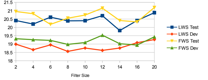
Fig. 10. Effects of different filter sizes on Phone Error Rate (PER in %) for LWS and FWS. The convolution and pooling plys use a pooling size of 6, shift size of 2, 150 feature maps for FWS, and 80 feature maps per frequency band for LWS.
