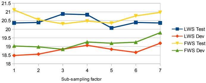
Fig. 8. Effects of different CNN shift sizes on Phone Error Rate (PER in %) for LWS and FWS. The convolution and pooling plys use a pooling size of 6, filter size of 8, 150 feature maps for FWS, and 80 feature maps per frequency band for LWS.
