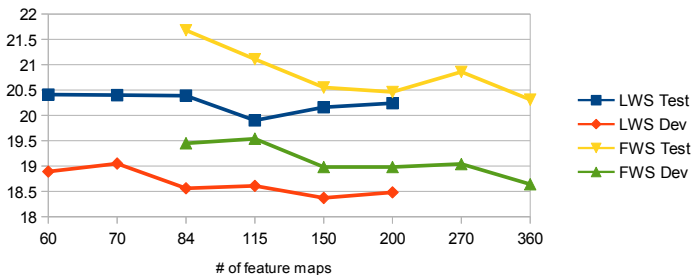
Fig. 9. Effects of different numbers of feature maps on Phone Error Rate (PER in %) for LWS and FWS. The convolution and pooling plys used a pooling size of 6, shift size of 2, filter size of 8.
