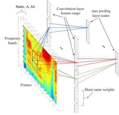
Fig. 5. An illustration of a CNN with limited weight sharing. 1-D convolution is applied along the frequency bands.
