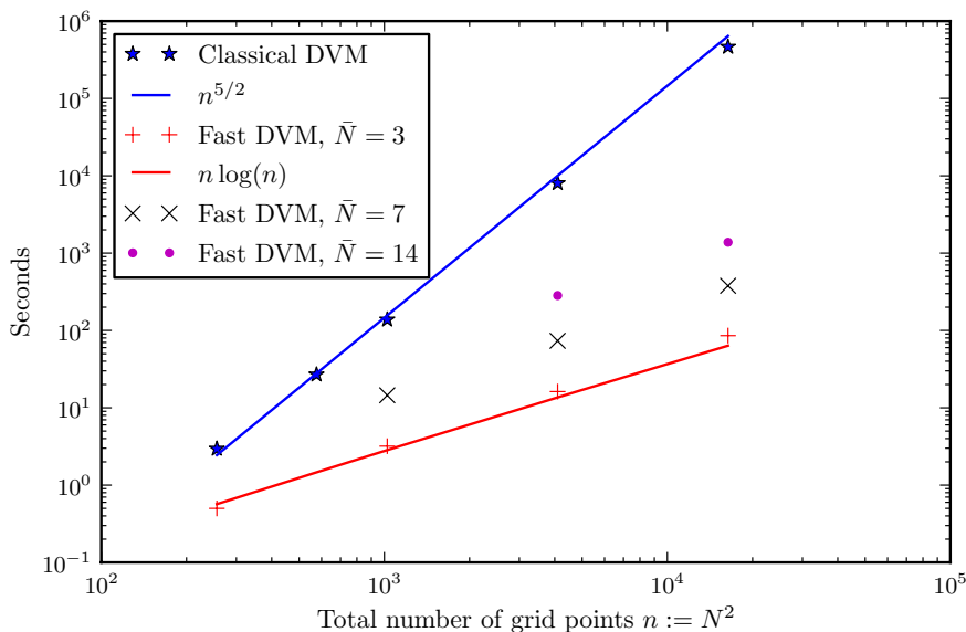
FIGURE 3. Evolution of the computational time with respect to the total number of points for the classical and fast DVM methods, at time T = 1 .
