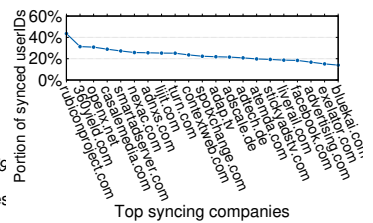
Figure 15: Portion of synced userIDs learned per tracker: 3 trackers learn more than 30% of the total userIDs in our dataset; 14 trackers learn more than 20% each.
