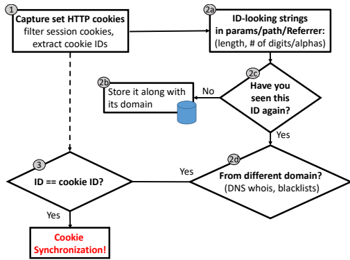
Figure 3: Heuristics-based CSync detection mechanism.
