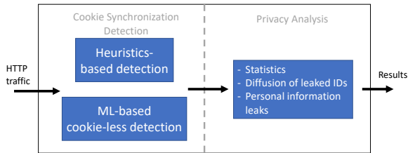
Figure 2: High-level overview of CONRAD’s internal components.
