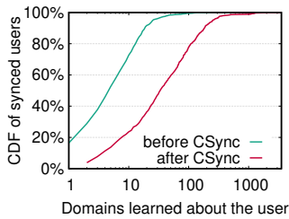
Figure 12: Distribution of domains learning at least a userID of a user (with/without the effect of CSync). After syncing, the domains that learned about the user grew by 6.75x.
