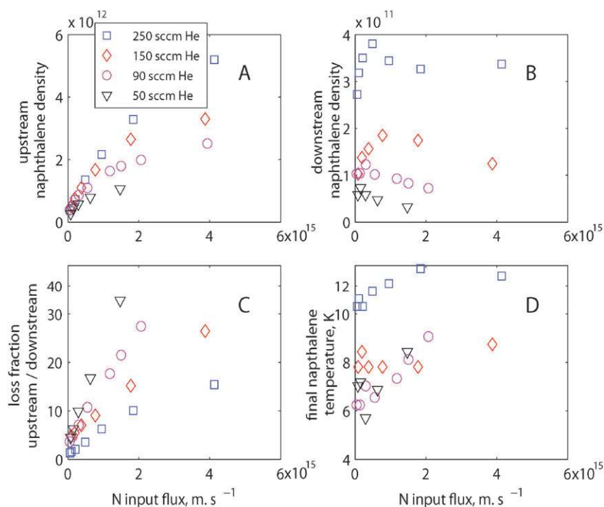
Fig. 3 Densities and temperatures of cold naphthalene under various conditions. Most of the cold naphthalene is lost as it is swept from the tube input ('upstream', subplot A) to the tube center ('downstream', subplot B). Loss in the tube (subplot C) clearly rises with increasing naphthalene input flux. The downstream temperature (subplot D) is in reasonable thermodynamic equilibrium with the cold ( \approx 6.5 K) cell for all but the highest helium flow rates.
