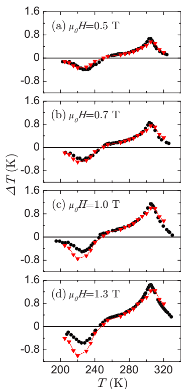
FIG. 4. (Color online) Adiabatic temperature change, as a function of temperature, for different magnetic fields. Circles stand for measured data and triangles correspond to data indirectly computed using equilibrium thermodynamics relationships.
