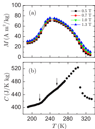
FIG. 3. (Color online) (a) Temperature dependence of the magnetization for selected values of the magnetic field. (b) Specific heat as a function of temperature. Arrows indicate the region of the reverse martensitic transition.
