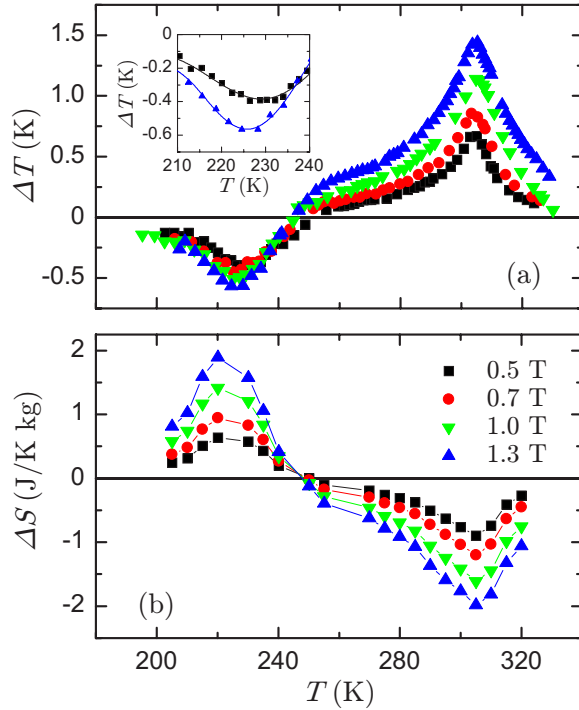
FIG. 2. (Color online) (a) Measured adiabatic temperature change and (b) computed isothermal entropy change, as a function of temperature at selected values of the magnetic field. The inset shows an enlarged view for the 0.5 and 1.3 T fields which illustrates the shift in the inverse MCE with magnetic field.
