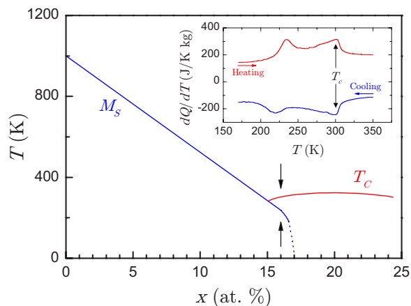
FIG. 1. (Color online) Phase diagram of \text{Ni}_{50}\text{Mn}_{50-x}\text{In}_x , obtained using the data in Ref. 11. M_S indicates the martensitic transition line and T_C indicates the Curie point line. The inset shows DSC curves for heating and cooling runs for the x=16 sample.
