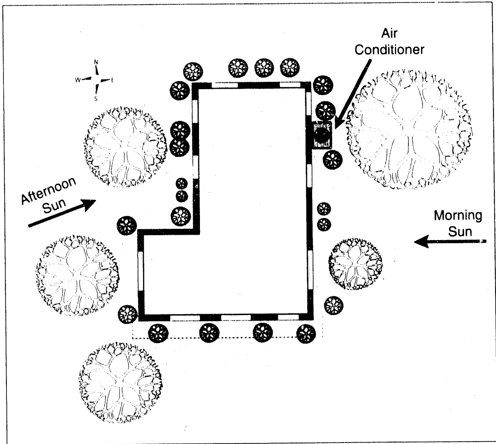
Figure ES-4. Sample residential landscape: A large tree is planted on the east side to shade the air conditioner, and on the west and south sides to cast maximum shadows on the house. Shrubs planted on all sides of the house help to reduce the temperatures of soil and walls. (Also appears as Figure 6-9.)
