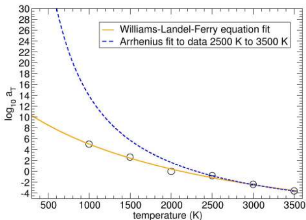
FIG. 9: (Color online) The log of the shift factor plotted vs the temperature. The data are fit two both Arrhenius and WLF theories. Error bars are smaller than the data points in the plot.
