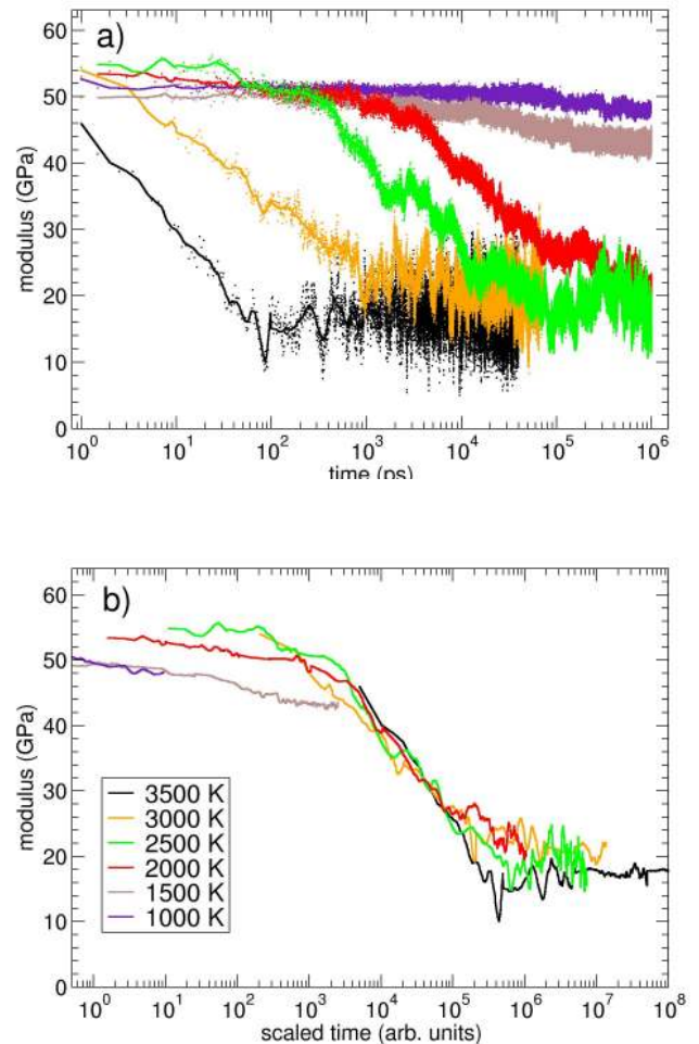
FIG. 7: (Color online) (a) The bulk stress relaxation modulus plotted vs log time from picosecond to microsecond times for temperatures from 3500 to 1000 K. (b) The same data, smoothed and shifted horizontally, collapse to show the master curve for silica.
