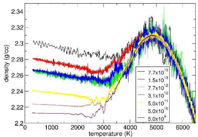
FIG. 1: (Color online) Plot of the density vs temperature for seven glass quenches completed with linear cooling rates, \gamma , ranging from 7.7 \times 10^{13} down to 5 \times 10^9 . All quenches qualitatively capture silica's anomalous density. Density, \rho(T) , is independent of ramp rate down to approximately 4500 K.
