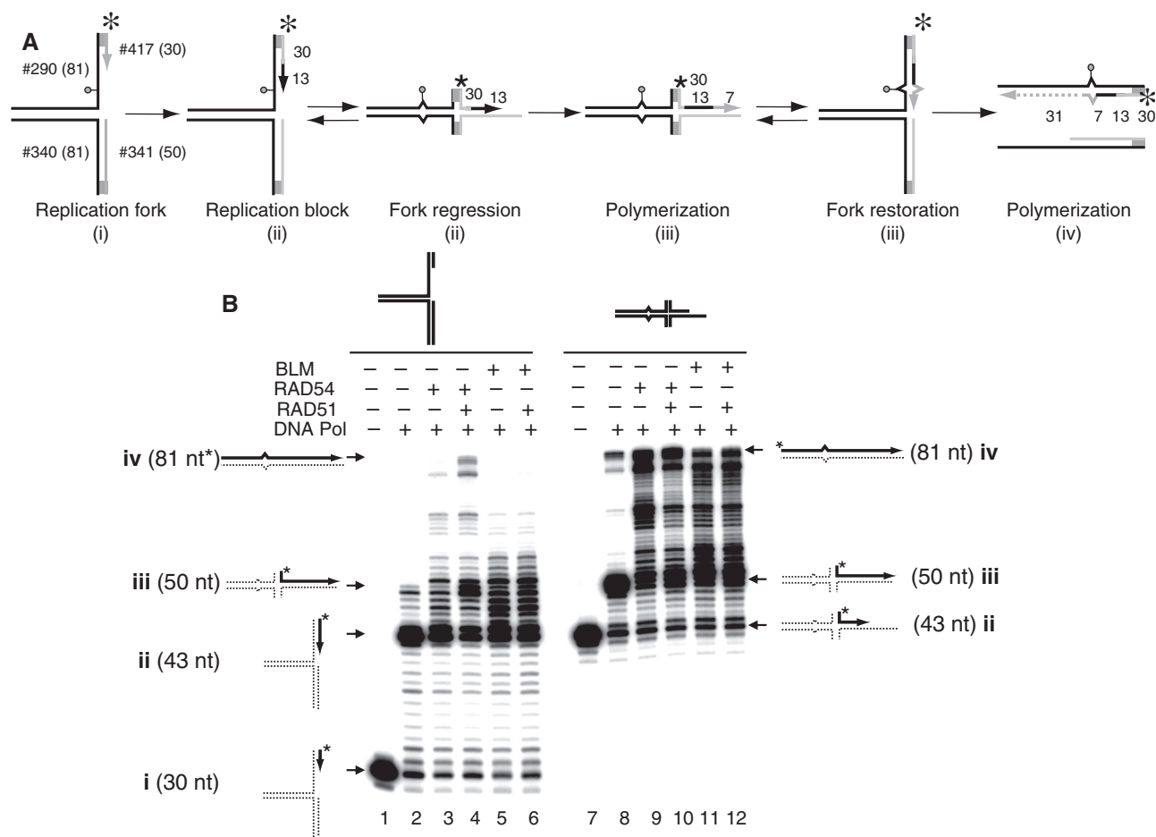
Figure 6. In vitro reconstitution of the DNA lesion bypass through the template switch mechanism. (A) The scheme of the lesion bypass via a mechanism that involves fork regression, DNA synthesis using the resulted chicken foot structure as a template, and fork restoration. The circle indicates the position of iso-C that mimics a DNA lesion at the stalled replication fork. The asterisk indicates the ^{32}\text{P} -label. Shaded regions denote heterologous DNA terminal branches that prevent complete strand separation during fork regression. The numbers indicate the numbers and length (nt) of the DNA fragments in the substrates and the products of the reaction. (B) DNA polymerase reactions were carried out using DNA polymerase I Klenow Fragment (10 ng/ml) and the replication fork (#290/417* + #340/341) (32 nM, molecules) (left) or the chicken foot structure (#341/342* + #340/290) (32 nM, molecules) (right) as templates. RAD54 (100 nM), BLM (50 nM) and RAD51 (200 nM) were added to the reactions as indicated in 'Materials and Methods' section. The products of DNA synthesis were analyzed by electrophoresis in a 15% denaturing polyacrylamide gel.
