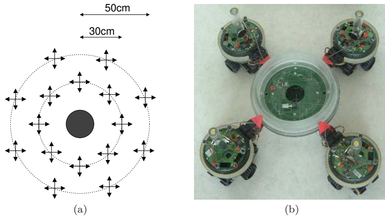
Fig. 6. (a) Potential starting points and orientations of the s-bots around the prey . (b) Four s-bots connected in “star-like” formation around the prey .
