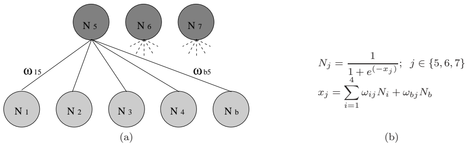
Fig. 7. (a) A graphical representation of the feed-forward two-layers artificial neural network of the assembly module. N_1, N_2, N_3 , and N_4 are the nodes which receive input from the s-bots sensors. N_b is the bias term. N_5, N_6 , and N_7 are the output nodes. (b) The equations used to compute the network output values.
