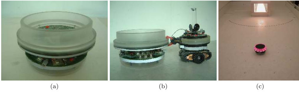
Fig. 5. (a) The prey . (b) An s-bot connected to the prey . (c) Overview of the arena with the prey located at a distance of 225 cm from a light bulb which represents the centre of a circular target zone.
