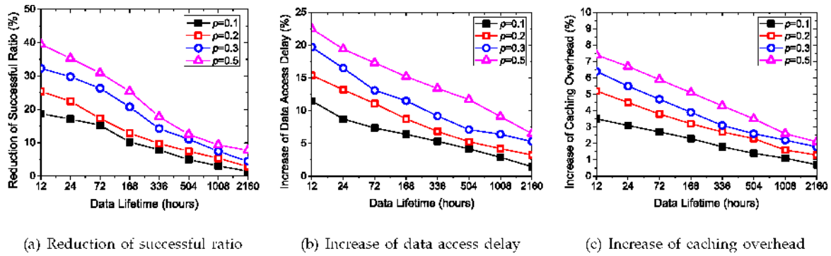
Fig. 17. Impact of NCL load balancing on the caching performance.
