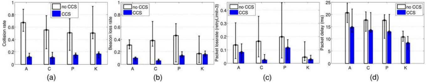
Fig. 17. TDMA performance of a ZigBee WPAN when it coexists with a WiFi WLAN. The x -axis denotes four different WiFi AP locations. Bars denote the performance averaged over all ZigBee links. Error bars denote the maximum and minimum values. Performance metrics include: (a) collision rate, (b) beacon-loss rate, (c) packet-loss rate, and (d) packet delay.
