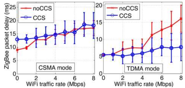
Fig. 16. Packet delivery delay (retryLimit = 3).
