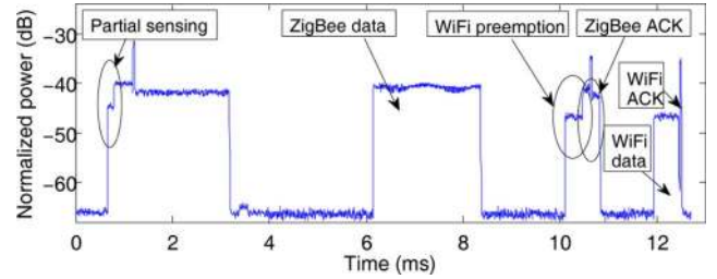
Fig. 6. Temporal collision hazards captured in the traces of a GNU-Radio/USR2 oscilloscope.
