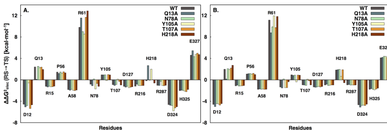
Figure 8. Electrostatic contribution of key residues to the calculated activation barrier for group transfer reactions of (A) PPP and (B) PET for different R1PMH variants.
