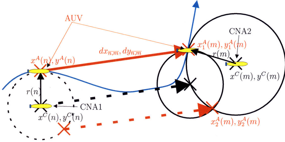
Figure 3-7: Computing two possible positions of the AUV at t(m) (x_1^A(m), y_1^A(m)) and (x_2^A(m), y_2^A(m)) using the dead-reckoning information dx_{\bar{n},\bar{m}}, dy_{\bar{n},\bar{m}} and the information x^C(n), y^C(n) and r(n) received at t(n) from CNA1 and x^C(m), y^C(m) and r(m) received at t(m) from CNA2.
