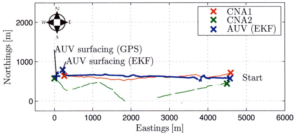
Figure 3-6: Setup and results of the AOFNC2003 MLBL experiment. Top: Setup. Two boats outfitted with GPS and LBL beacons and an AUV (with DVL and compass) interrogating both beacons. Bottom: GPS-track of the boats (CNAs) and the AUV's position estimate using an EKF. Note the difference between the estimated ( \times ) and the true surfacing position (+).
