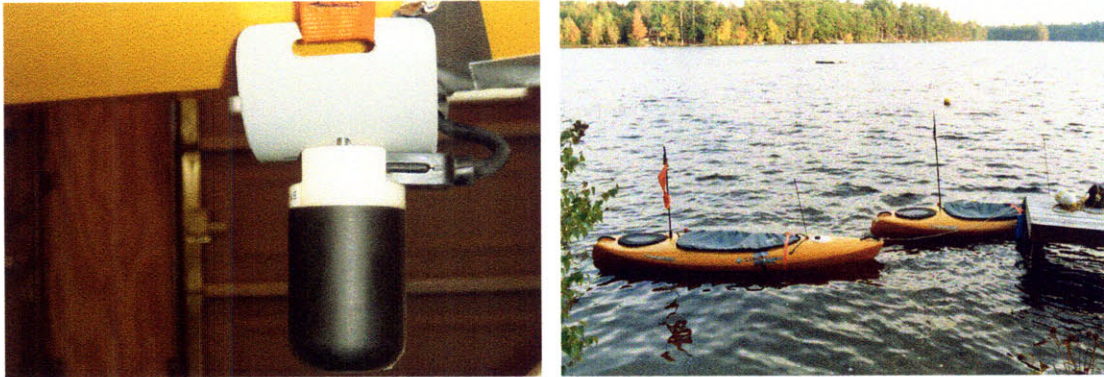
(a) Modem transducer strapped to the hull (b) Two kayaks moored on the pier while the a third one moves and determines its distance to the moored ones using the acoustic modem
