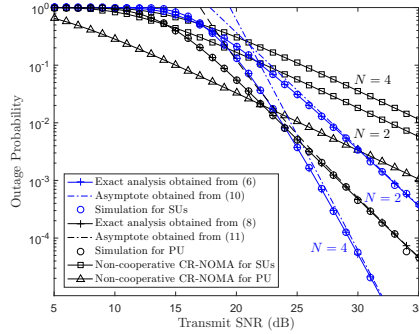
Fig. 1. Outage probability for the primary and secondary systems versus transmit SNR.
