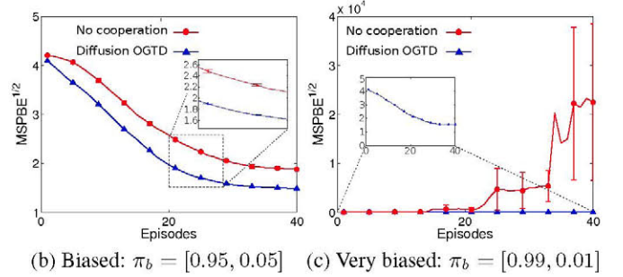
Fig. 1. Taxi example. (a) State diagram, and (b)-(c) mean-square-projected-Bellman-error (MSPBE) for a target policy \pi = [0.2, 0.8] , estimated by 10 cooperative versus 10 non-cooperative agents. In (b), though we see some improvement in the cooperative agents, non-cooperative agents are still good at finding the estimate. In (c), when the behavior policy is very biased, there is a clear benefit of diffusion: while non-cooperative nodes diverge, cooperative agents achieve a good stable estimate. The feature vectors for states 13, 9, 5 and 1 are x(13) = [1, 0, 0, 0]^\top , x(9) = [0, 1, 0, 0]^\top , x(5) = [0, 0, 1, 0]^\top and x(1) = [0, 0, 0, 1]^\top respectively, for the rest of states, the features are obtained interpolating linearly between these (i.e., x(2) = [0, 0, 1/4, 3/4]^\top , x(3) = [0, 0, 1/2, 1/2]^\top , x_4 = [0, 0, 3/4, 1/4]^\top , and so on). Step-sizes are constant \mu = 0.1 and \eta = 10 . The combination coefficients of the estimates, B , are obtained using the Metropolis method [13]. Finally, P_{\text{mov}}(\text{exit}) = 0.8 , \forall s \in \mathcal{S} , and P_{\text{mov}}(s, \text{motorway}) = e^{-\frac{s-13}{13}} , s \in \mathcal{S} .
