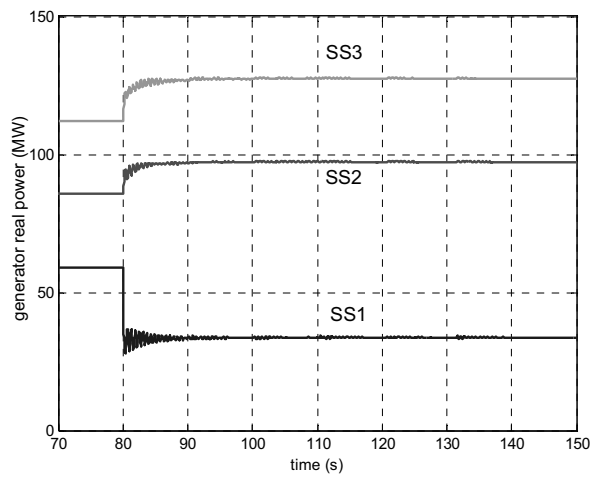
Figure 9 Response of Generator Real Power – Case 1
