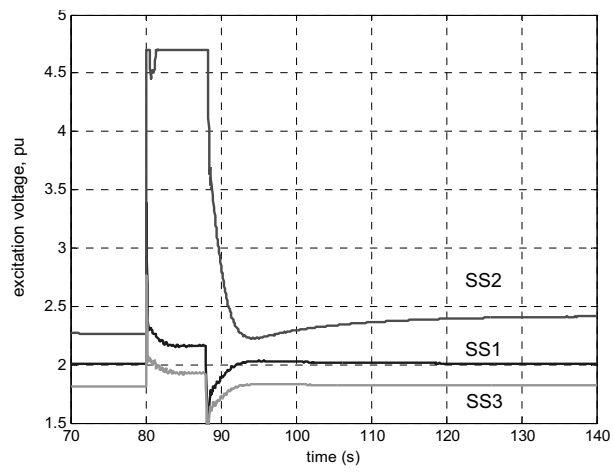
Figure 14 Response of Generator Excitation Voltages (pu) – Case 2
