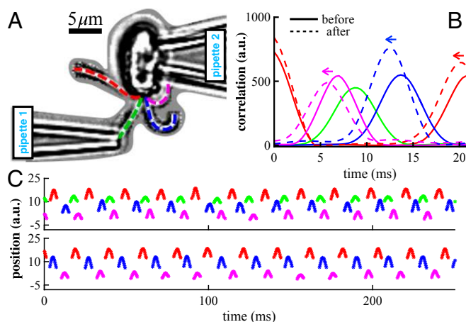
Fig. 4. (A) Stalling the flagellum beat in T. suecica . (B) Beat correlations for each flagellum relative to a reference flagellum (red) computed before and after manipulation shows period shift but no change in the order of flagella actuation. (C) Timeseries or footprints delineate positions of flagella (labeled as in A) before (Top) and after (Bottom) manipulation.
