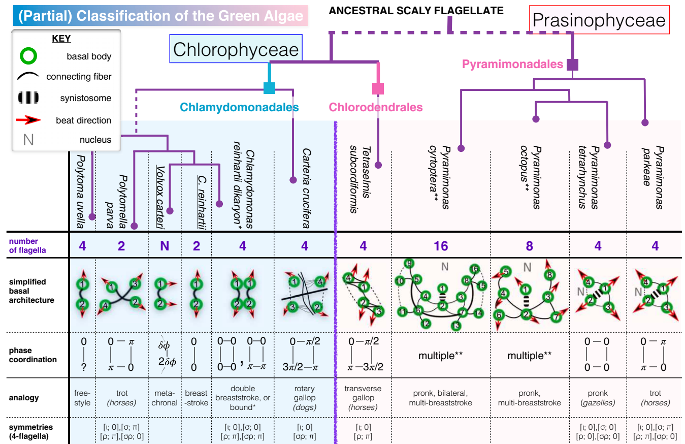
Fig. 5. Algal species are compared in terms of phylogeny, number and orientation of flagella, arrangement of BBs/basal architecture (see also SI Appendix), and patterns of coordination defined by the relative phases between flagella. Vertical lines approximate the relative phylogenetic distance from a putative flagellate ancestor (SI Appendix) (only partial branchings are shown). Free-swimming quadriflagellate gaits are readily identified with quadruped locomotion, revealing the symmetries of an underlying oscillator network. Asterisk (*): Quadriflagellate dikaryons of CR gametes perform a double breaststroke gait with the same symmetries as the pronk (Movie S5), but this gives way to a bound gait when both sets of flagella undergo phase slips simultaneously. Double asterisk (**): See Movies S7 and S8.
