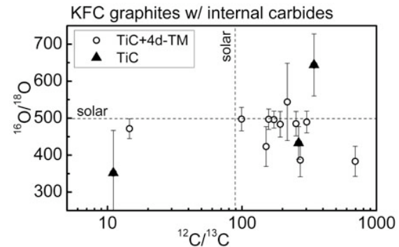
Figure 2. C and O isotopic ratios of graphites which contain either 1) (Ti,Zr,Mo,Ru)C solid-solution carbides or 2) pure TiCs (no Zr, Mo, or Ru).
